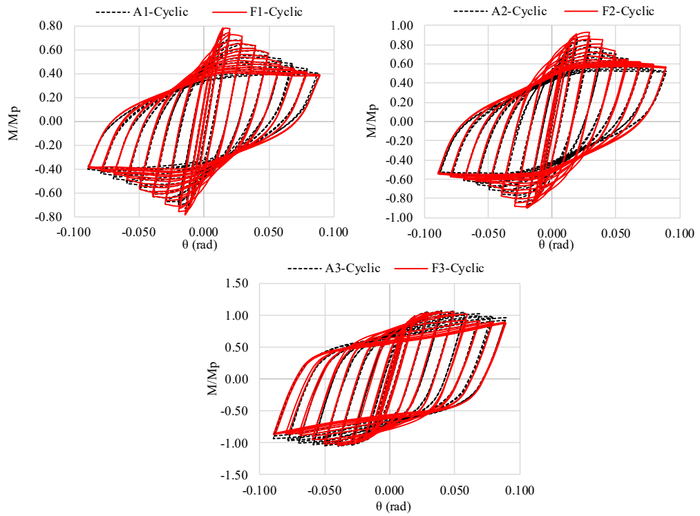
Fig. 5. Moment-Rotation curves for FE numerical models
