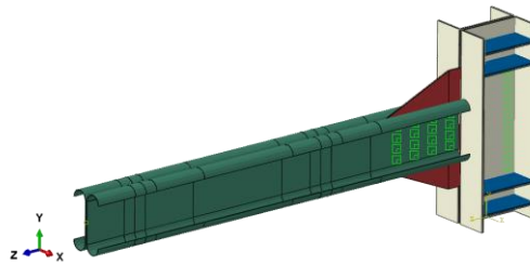
Fig. 1. General 3D view of the connection model
