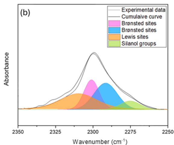
Fig. 5. FT-IR spectra of ZSM-5 (117): (a) OH-stretching region ( 3800\text{--}3200\text{ cm}^{-1} ) after thermal pretreatment and during \text{CD}_3\text{CN} adsorption at increasing pressures ( 6 \times 10^{-1}\text{ mbar} and 16 mbar); (b) \text{C}\equiv\text{N} stretching region ( 2350\text{--}2250\text{ cm}^{-1} ). FT-IR spectra for the other zeolites are reported in Fig. S6.
