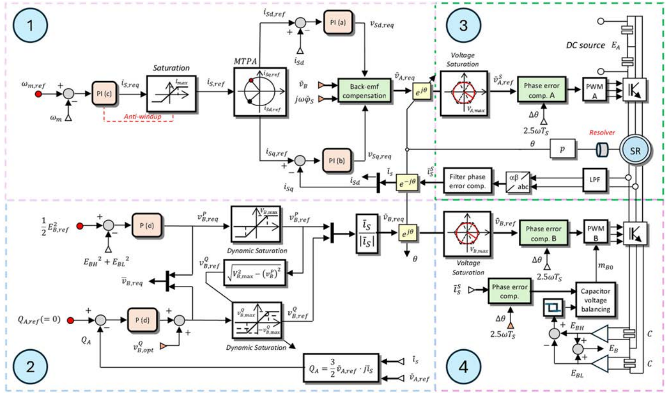
FIGURE 26. Overall control architecture of the proposed TURBO open-end winding SynRM drive.
