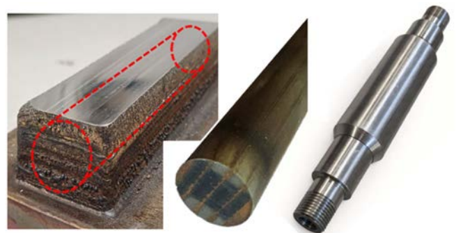
FIGURE 8. Fabrication sequence: as-built multilayer block, intermediate cylindrical preform, and finish-machined rotor.
