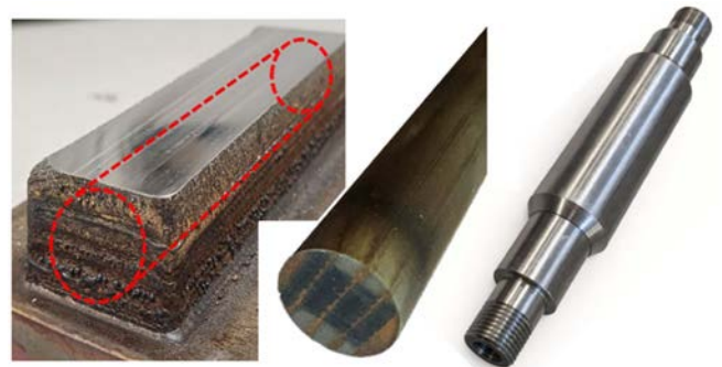
FIGURE 8. Fabrication sequence: as-built multilayer block, intermediate cylindrical preform, and finish-machined rotor.
