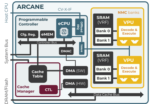
Figure 1: ARCANE block diagram in a two-VPUs, two-lanes configuration
