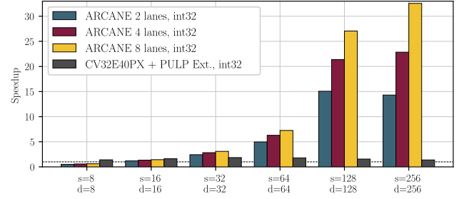
Figure 4: Relative speedup with 2-,4-,8-lane configuration of ARCANE and cv32e40px on int32 compared to cv32e40x when running the FWSA layer.
