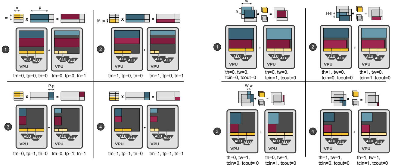
Figure 2: Complete Matmul (left) and single output channel of a Conv2D(right) mapping and tiling on ARCANE VPU.
