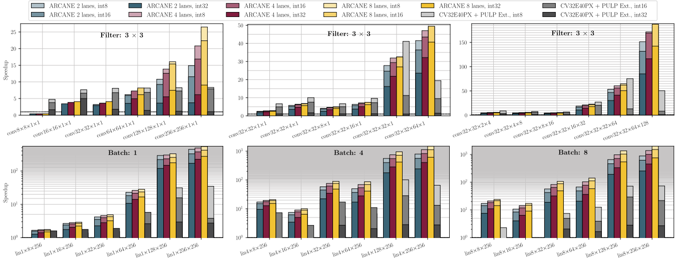
Figure 3: Relative speedup improvements with 2-, 4-, 8-lane configuration of ARCANE and cv32e40px on int8, int16, int32 compared to cv32e40x when running (Top) 2D Convolution ( convH \times W \times C_{in} \times C_{out} ) with a 3 \times 3 filter and (Bottom) Matrix Multiplication ( linB \times (X_{cols} | W_{rows}) \times W_{cols} ).
