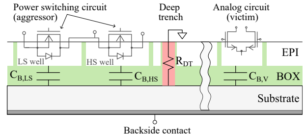
Fig. 1. Cross-section of an SOI smart power IC.
