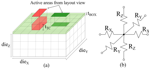
Fig. 2. (a) 3D structure discretized according to FDM model, and (b) electrical equivalent of elementary parallelepiped.
