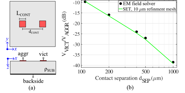
Fig. 5. (a) Two-contacts structure and (b) corresponding results in terms of aggressor to victim transfer function.
