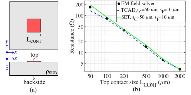
Fig. 4. (a) Simulated structure and (b) extracted spreading resistance by different tools for the one-top contact.
