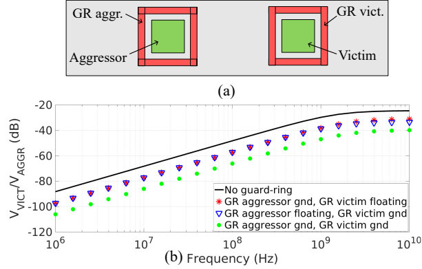
Fig. 7. (a) Two-contacts structure with guard-rings and (b) corresponding results in terms of aggressor to victim transfer function as a function of guard rings connection.
