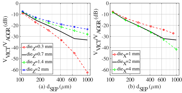
Fig. 6. Sweep of (a) die thickness and (b) die width for the two-contact structure shown in Fig. 5(a).
