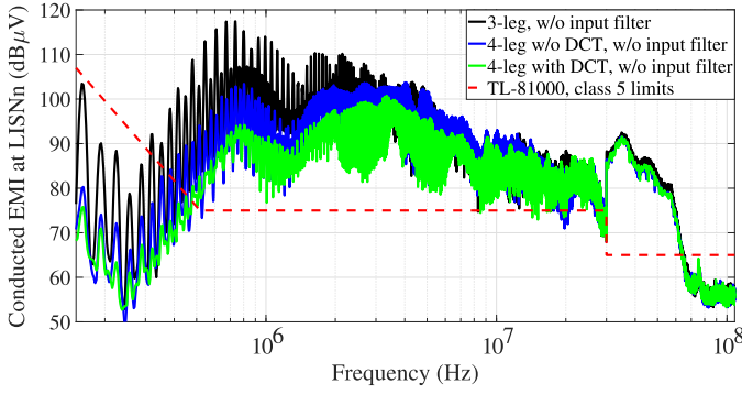
Fig. 11. Measured conducted EMI for three-leg VSI with SVM (black), four-leg VSI without (blue) and with (green) DCT applied.
