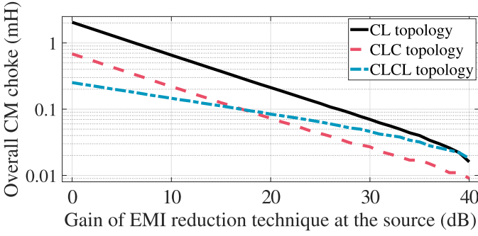
Fig. 4. Required inductance for CL (solid), CLC (dashed) and CLCL (dashed-dot line) input filter as a function of the G_{dB} achievable by adopting a CM EMI reduction technique at the source.
