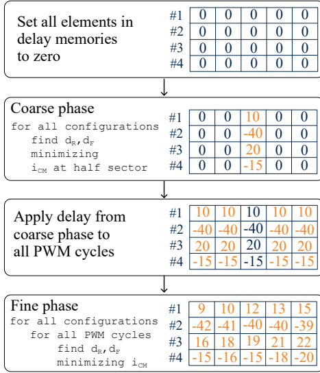
Fig. 8. Flowchart of the proposed algorithm to populate the delay LUTs shown in Fig. 7.
