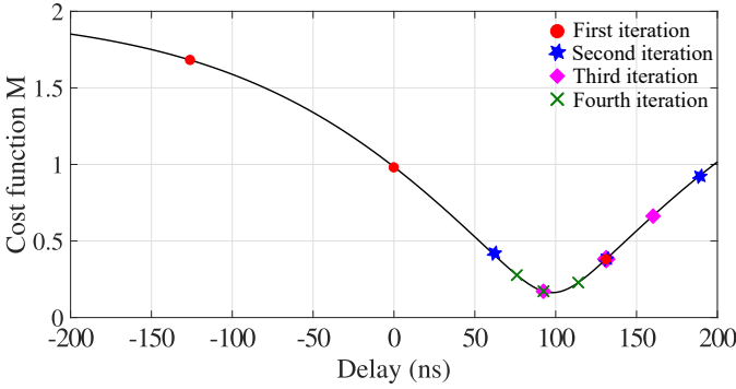
Fig. 9. Ternary search algorithm to determine the optimal delay in two complementary switching legs.
