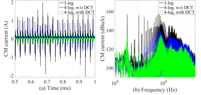
Fig. 10. Measured CM current in (a) time-domain and (b) frequency-domain for the prototype used as a conventional three-leg VSI (black), as four-leg with AZSPWM-3 without (blue) and with (green) the DCT applied.
