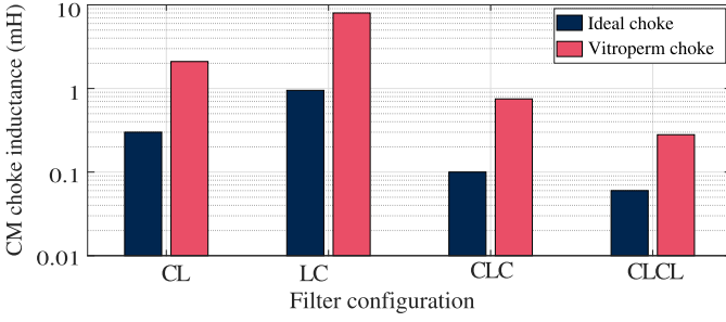
Fig. 3. Required inductance for different filter topology/number of stages with a constant Y-capacitance. Dark bars refer to ideal chokes, light bars to real chokes where permeability is frequency dependent.
