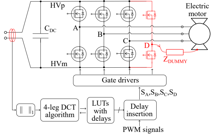
Fig. 7. Block scheme of the proposed solution to apply DCT to four-leg VSIs.
