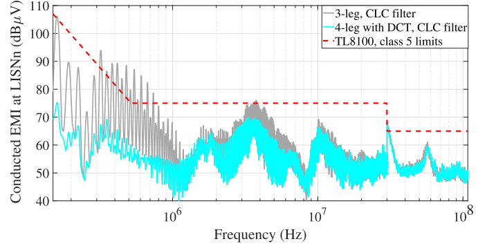
Fig. 12. Measured conducted EMI with the CLC filter inserted for the inverter operating as three-leg VSI with SVM (gray) and as a four-leg VSI with DCT applied (light blue spectrum).
