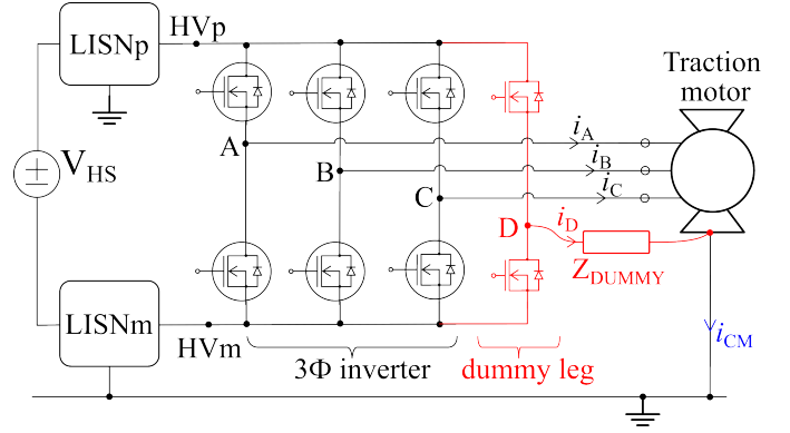
Fig. 5. Four-leg VSI driving a three-phase motor without the output filter. The fourth leg is connected to the dummy impedance Z_{DUMMY} to control the injected CM current.
