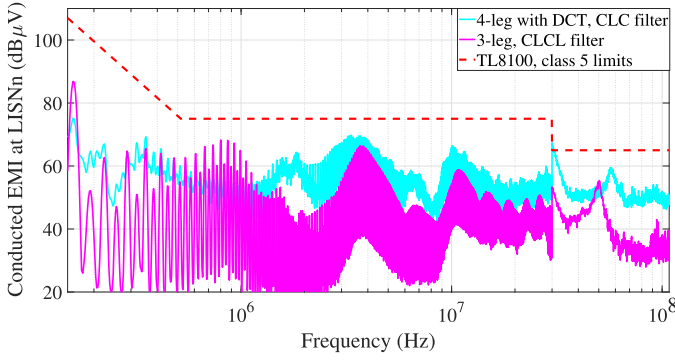
Fig. 13. Measured conducted EMI with the inverter operating as three-leg VSI with SVM and the CLCL filter (fucsia) and as four-leg VSI with DCT and CLC filter (light blue spectrum).
