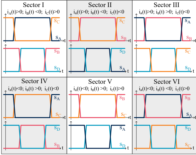
Fig. 6. Control signals of the four legs according to AZSPWM-3 for the six sectors.
