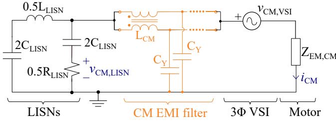
Fig. 1. CM EMI model of a motor drive system. The input EMI filter is placed between the LISNs and the device under test, i.e., the inverter and the motor.
