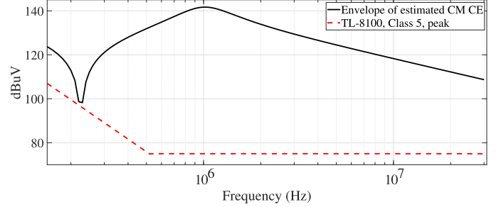
Fig. 2. Estimated envelope of CM EMI for a traction motor drive (solid) based on the values reported in Tab. I.
