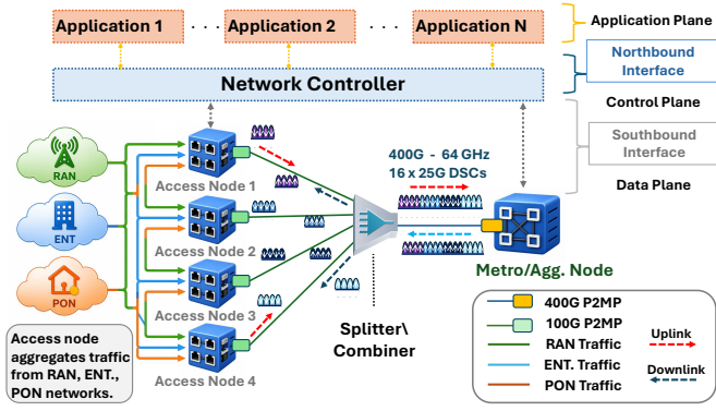
Fig. 2. Filterless P2MP converged metro-access architecture.
