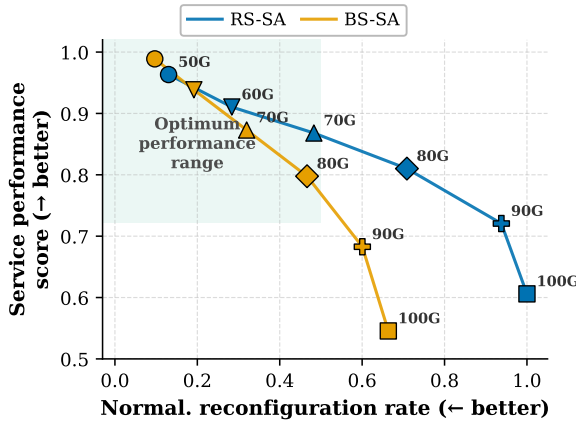
Fig. 8. Service performance versus normalized reconfiguration rate for RS-SA and BS-SA.
