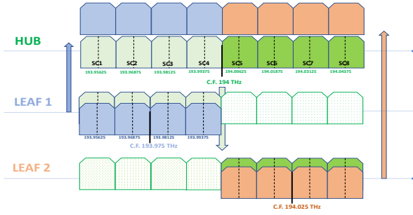
Fig. 1. DSCM enabled independent SCs on a single shared wavelength, where upstream and downstream transmissions are separated by slight offsets in central frequency to enable di-directional transmission.
