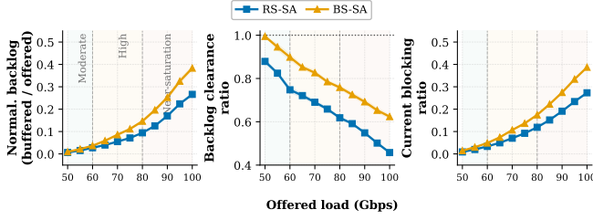
Fig. 5. Backlog dynamics versus offered load: normalized backlog, clearance ratio, and blocking ratio.
