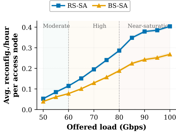
Fig. 7. Average subcarrier reconfiguration rate versus offered load for RS-SA and BS-SA.
