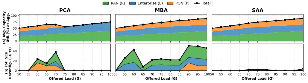
Fig. 4. Allocation policies performance at the hub/agg. node for different offered loads: row (a) : avg. capacity utilization (%) across 10 timestamps; row (b) : tot. SCs reconfigurability across all access nodes.
