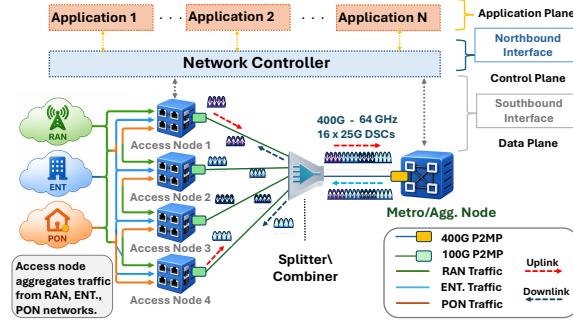
Fig. 1. Filterless P2MP converged metro-access network
