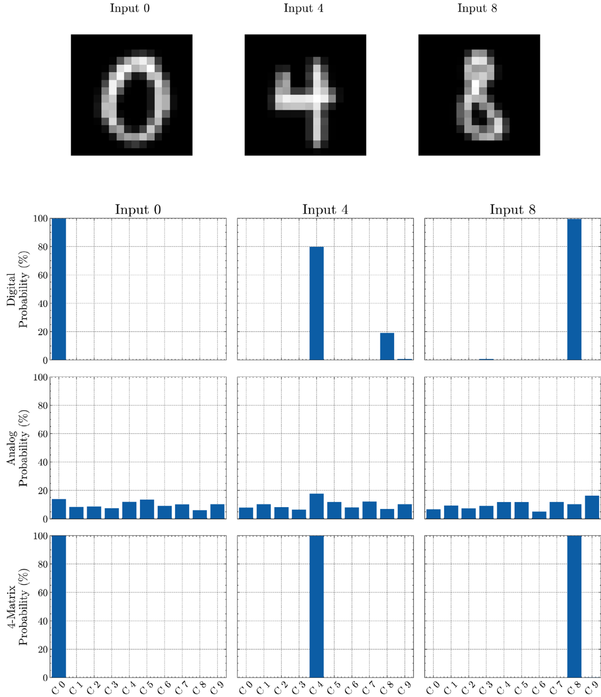
FIGURE 5 | MLP inference results with four-matrix compensation. (a) MNIST input images used for inference. Representative input samples corresponding to digits 0, 4, and 8, resized to 16 \times 16 pixels and used as inputs to the multi-layer perceptron. (b) Corresponding output class probability distributions for digital, analog, and compensated analog MVM. Each column corresponds to a fixed input digit, while rows report the three computational modalities.
