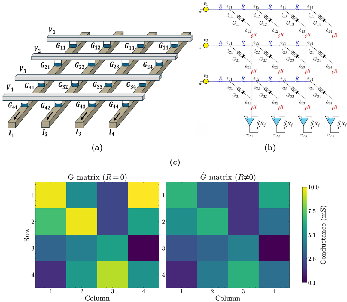
FIGURE 1 | Crossbar operation, circuit implementation, and effect of wire resistance. (a) A 4 \times 4 memristive crossbar highlighting the technical operating principle. (b) Circuit implementation: schematic of an m \times n memristive crossbar ( m \neq n ) with wire resistance R to emphasize generality beyond square arrays. (c) Impact of wire resistance: the programmed conductances in the non-ideal case (second matrix, R \neq 0 ) are degraded relative to the ideal case (first matrix, R = 0 ). Results shown were obtained with the following simulation parameters: G_{\min} = 0.1 mS, G_{\max} = 10 mS, R = 5 \Omega , n = 4 .
