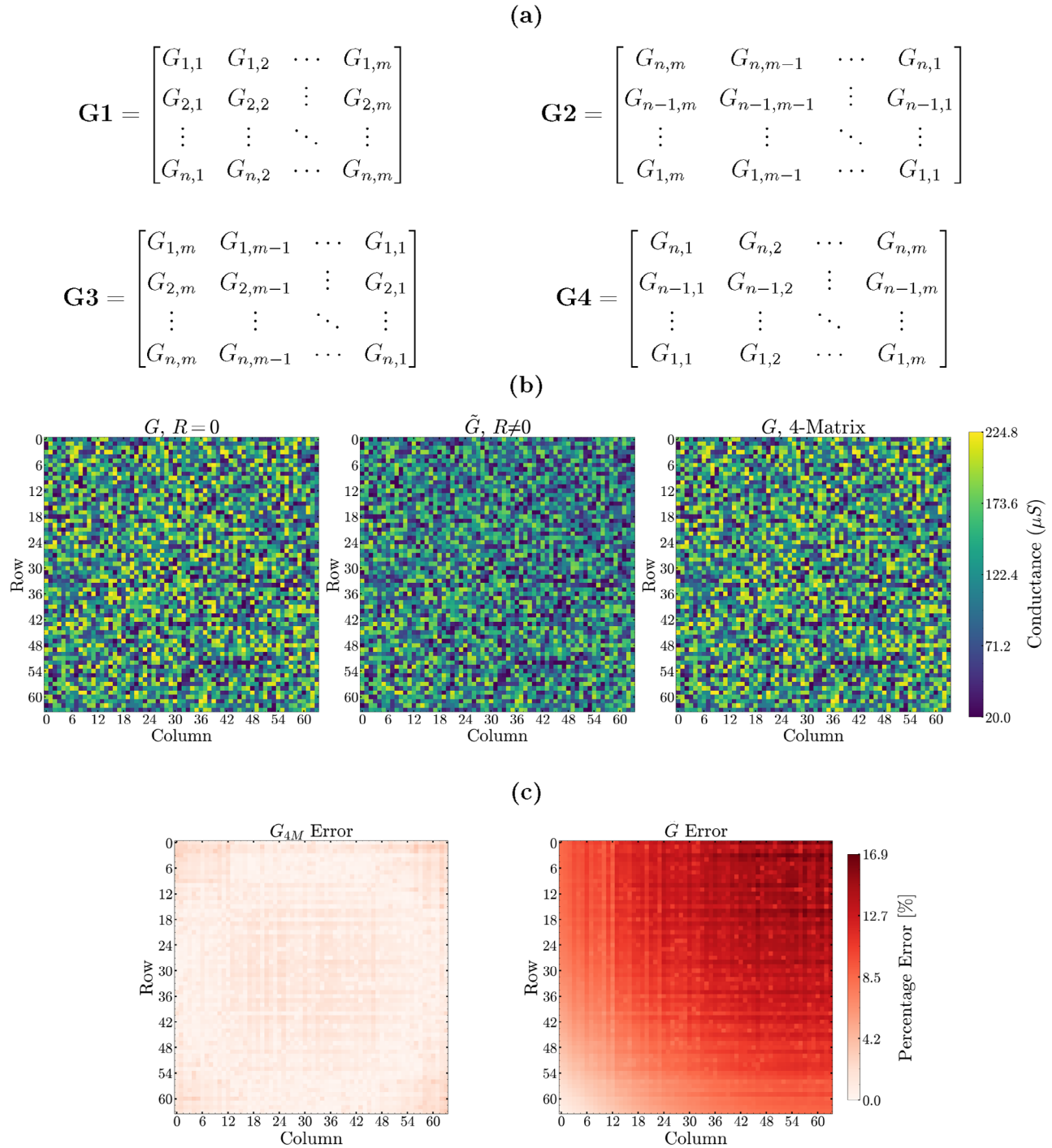
FIGURE 3 | (a) Geometric and symmetric transformations of the four matrices \mathbf{G1} , \mathbf{G2} , \mathbf{G3} , and \mathbf{G4} . (b) Left panel: original conductance matrix \mathbf{G} programmed in the crossbar. Middle panel: effective conductance matrix \tilde{\mathbf{G}} including wire resistance effects. Right panel: corrected conductance matrix obtained after applying the four-matrix method. (c) Percentage error associated with each memconductance in the crossbar for \mathbf{G_{4M}} and \tilde{\mathbf{G}} . Simulation parameters: G_{\min} = 20 \mu\text{S} , G_{\max} = 224.8 \mu\text{S} , R = 0.35 \Omega , n = 64 .
