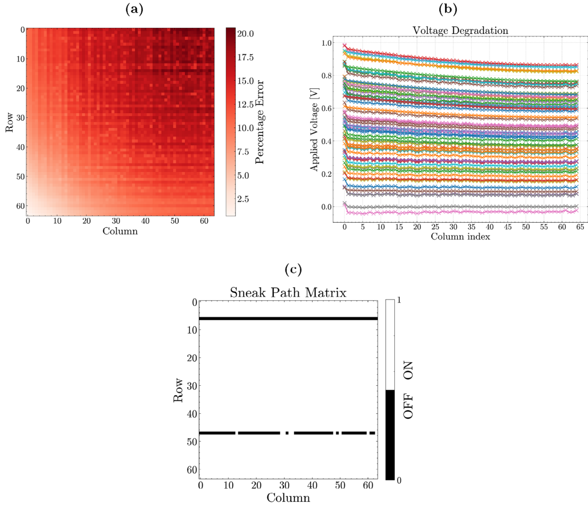
FIGURE 2 | | Error analysis, voltage degradation, and sneak path simulations in crossbar arrays. (a) Relative errors associated with the effective conductance matrix (simulation parameters: G_{\min} = 10 \mu\text{S} , G_{\max} = 100 \mu\text{S} , R = 1 \Omega , n = 64 ). (b) Degradation of voltages along a selected row of the crossbar. (c) Simulation of sneak path currents within the array.
