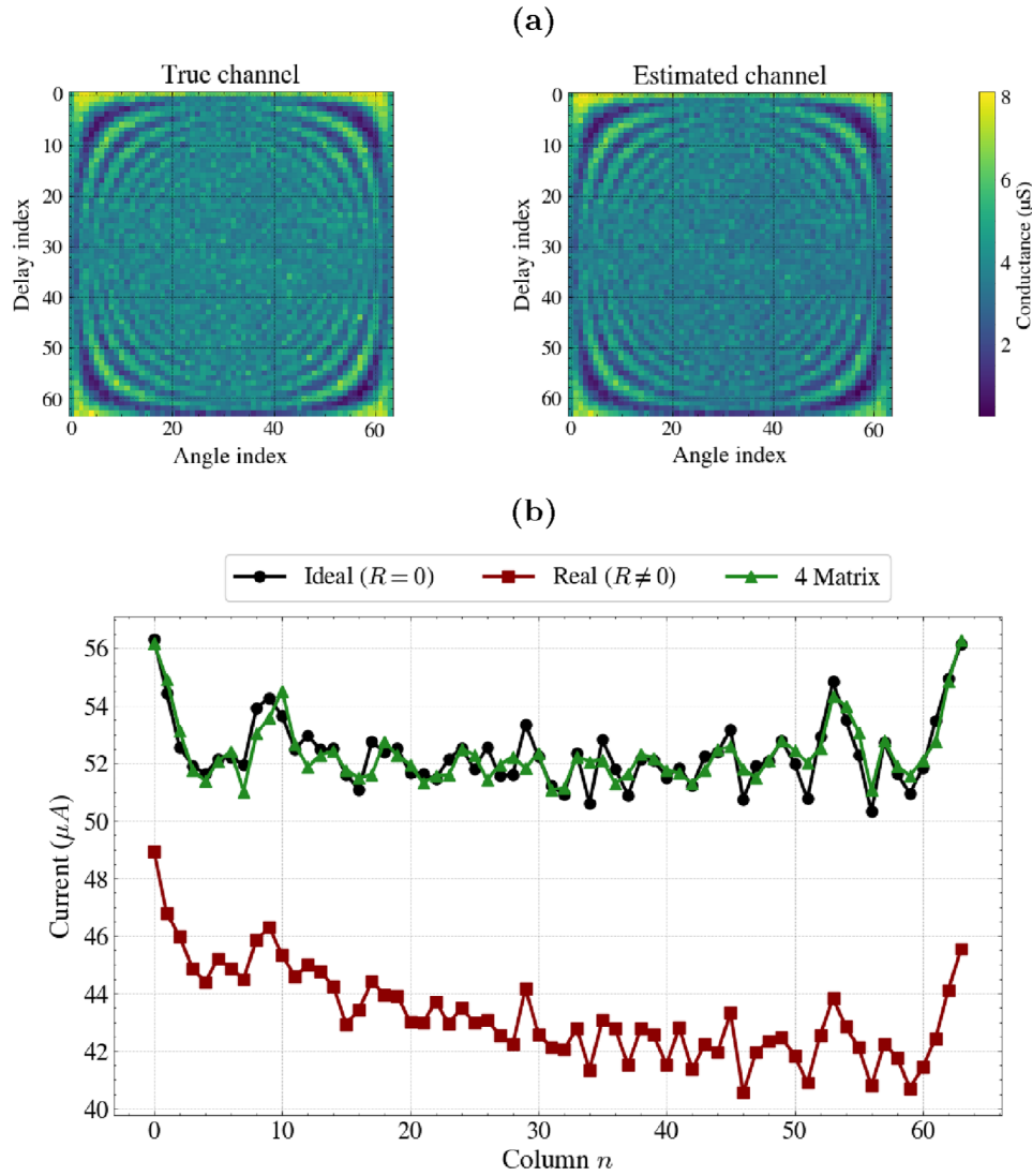
FIGURE 4 | DFT experimental implementation on the memristor crossbar. (a) Programmed real-valued 64 \times 64 DFT conductance matrix and measured dot product engine platform (Section S8) effective conductance map showing spatial distortion induced by line resistance. (b) Column-wise output currents for the ideal digital DFT ( R = 0 ), uncompensated hardware measurement ( R \neq 0 ), and four-matrix compensated output. The compensation substantially reduces frequency-domain distortion and suppresses error scaling with array dimension on real hardware.
