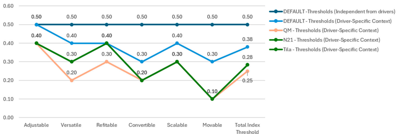
Figure 6. Threshold variation across scenarios (analysis of drivers).
