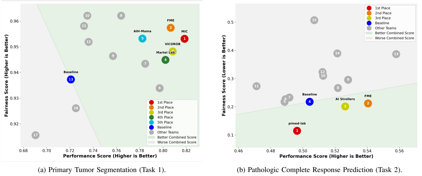
Fig. 1: Fairness plotted against performance across the two MAMA-MIA benchmark tasks. Teams with fairness-performance tradeoffs within the area indicated in green improve upon the baseline tradeoff. Note that the axis ranges are restricted to improve readability; consequently, teams falling outside these bounds are not shown.
