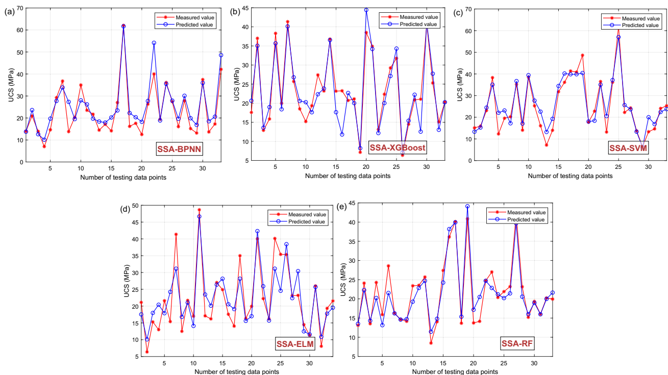
Fig. 6 UCS prediction performance of various models on the testing dataset: a SSA-BPNN, b SSA-XGBoost, c SSA-SVM, d SSA-ELM, e SSA-RF
