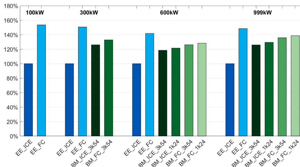
Fig. 5. Electrical Energy equivalent (EE equivalent) for all configurations, normalised to EE ICE configuration.
