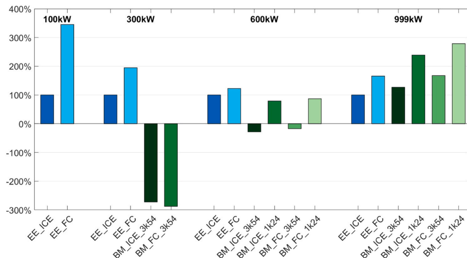
Fig. 7. NPV 15 for all plant configurations with respect to NPV 15 of EE_ICE configuration.
