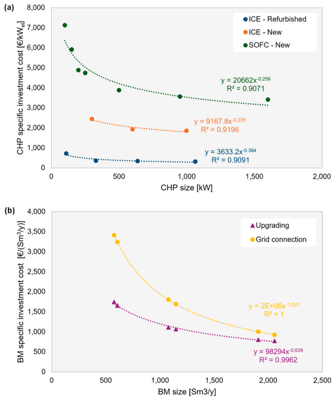
Fig. 3. (a) Specific capital cost of CHP technologies (refurbished ICE, new ICE and new SOFC) as a function of installed electrical capacity. (b) Specific capital cost of biomethane production systems (upgrading unit and gas grid connection) as a function of the annual biomethane production capacity. Dotted lines represent the fitted cost-size correlations derived from the investment data reported in Appendix A and in the Supplementary Material .
