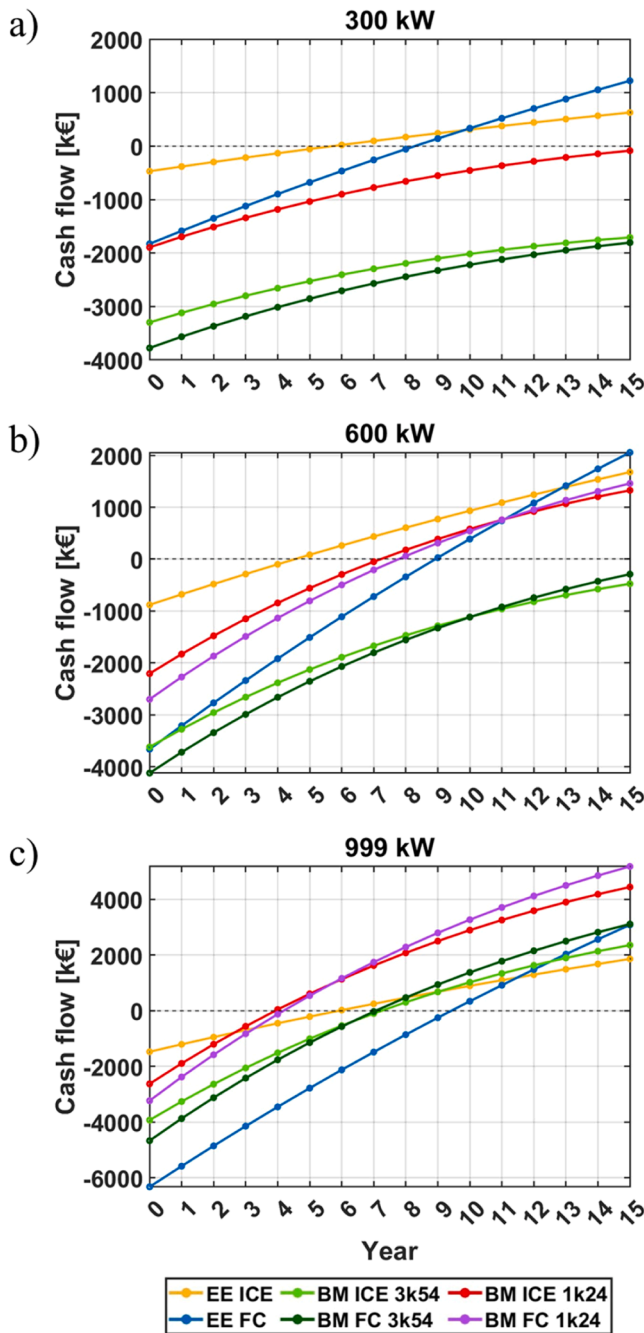
Fig. 6. Cumulative cash flows for all plant configurations.
