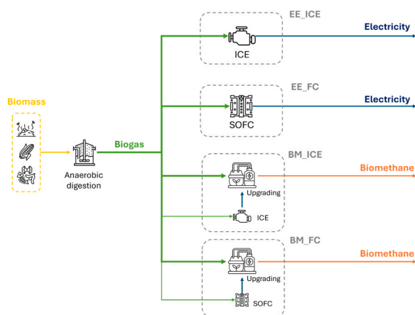
Fig. 1. Conceptual representation of the four technological pathways considered.
