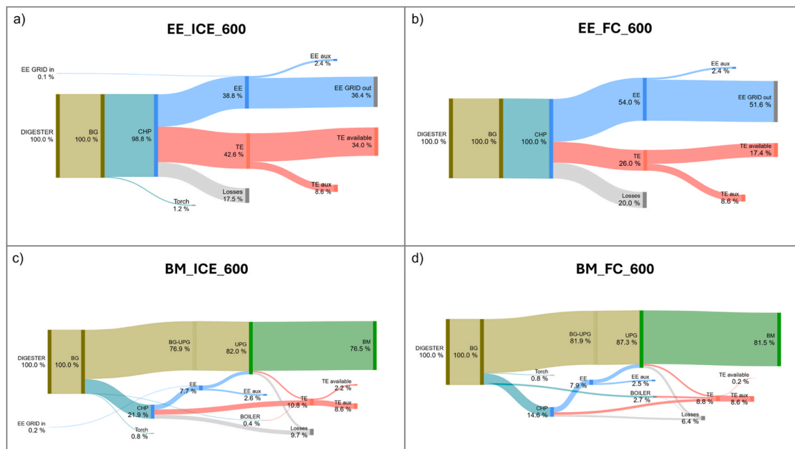
Fig. 4. Energy flow distribution for a) EE_ICE_600 configuration, b) EE_FC_600 configuration, c) BM_ICE_600 configuration, and d) BM_FC_600 configuration. All BM configurations refer to the 3k54 case.
