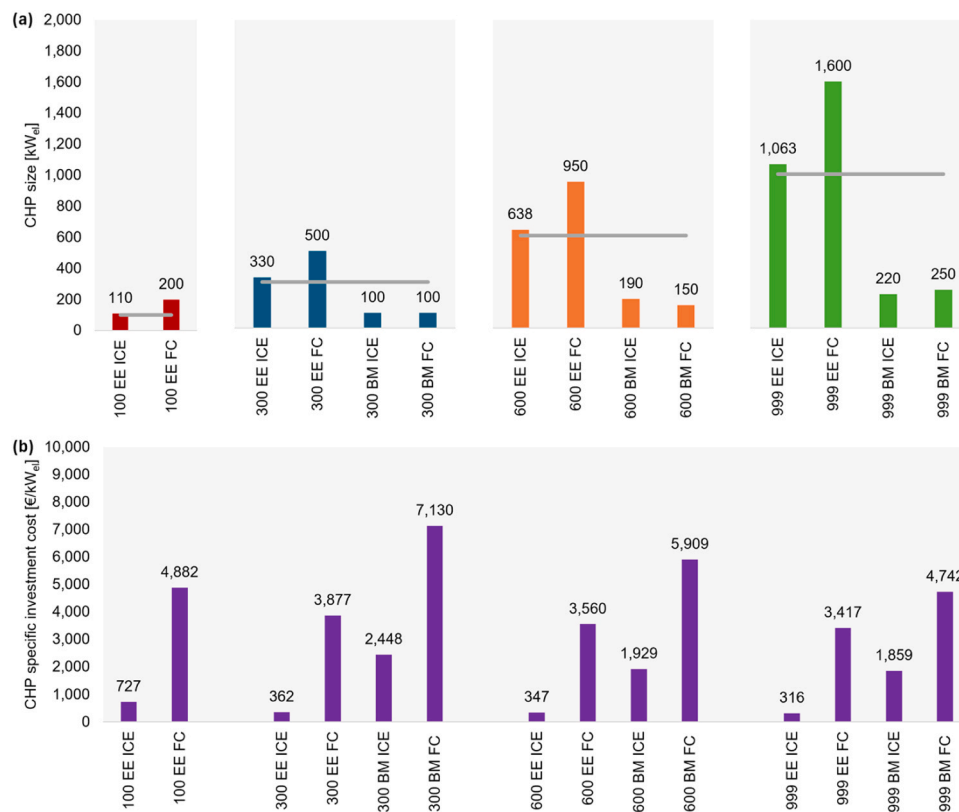
Figure A.1. (a) CHP size, evaluated for both EE and BM configurations. (b) CHP specific investment cost for the same system sizes and configurations
