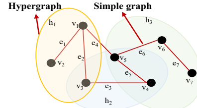
Fig. 2. Comparison of simple graph and hypergraph structure
