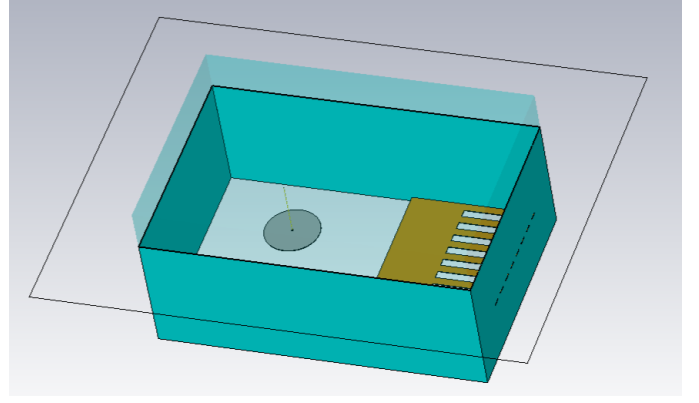
Fig. 2. CST Anechoic chamber geometry
