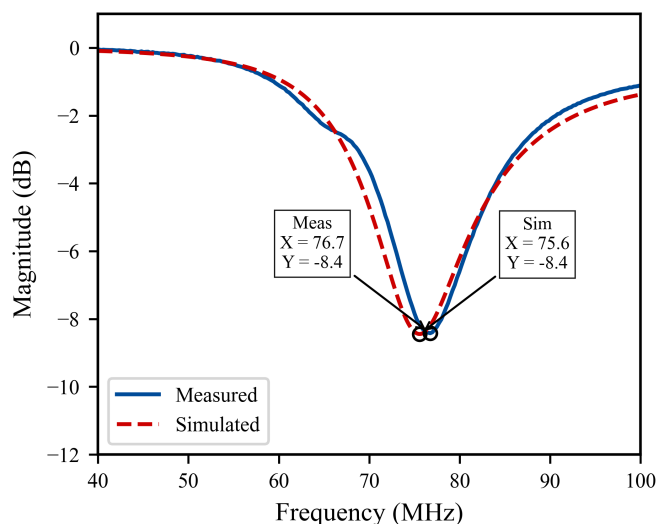
Fig. 4. Case study: S_{11} of a monopole antenna with circular ground plane.
