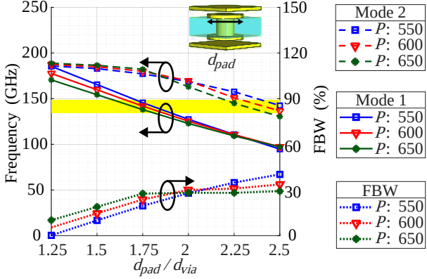
Fig. 4. Dispersion diagrams at d_{\text{via}} : 200 \mu\text{m} , h : 200 \mu\text{m} , g : 50 \mu\text{m} . (a) varying circular pad/via diameter ratios at different periods including fractional bandwidth. Yellow rectangle depicts the 134 – 148.5 GHz range. Inset: unit cell.
