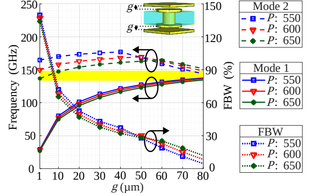
Fig. 6. Dispersion diagram for various gap sizes across a range of periods including fractional bandwidth. Yellow rectangle shows the 134–148.5 GHz range. Inset: unit cell. h : 200 \mu\text{m} , d_{\text{via}} : 200 \mu\text{m} , d_{\text{pad}} : 400 \mu\text{m} .
