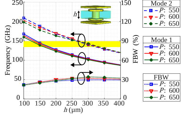
Fig. 5. Dispersion diagram for various substrate heights at different periods including fractional bandwidth. Yellow rectangle indicates the 134–148.5 GHz band. Inset: unit cell. d_{\text{via}} : 200 \mu\text{m} , d_{\text{pad}} : 400 \mu\text{m} , g : 50 \mu\text{m} .
