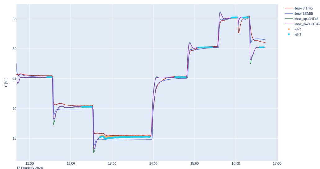
Figure 3. Time series of temperature readings from all sensors under test during the thermal characterization without the external case. The 25 °C set-point was repeated twice to assess reproducibility.
