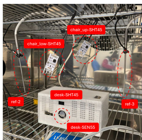
Figure 1. Experimental setup for the thermal characterization of the MIRABLE MS temperature sensors.
