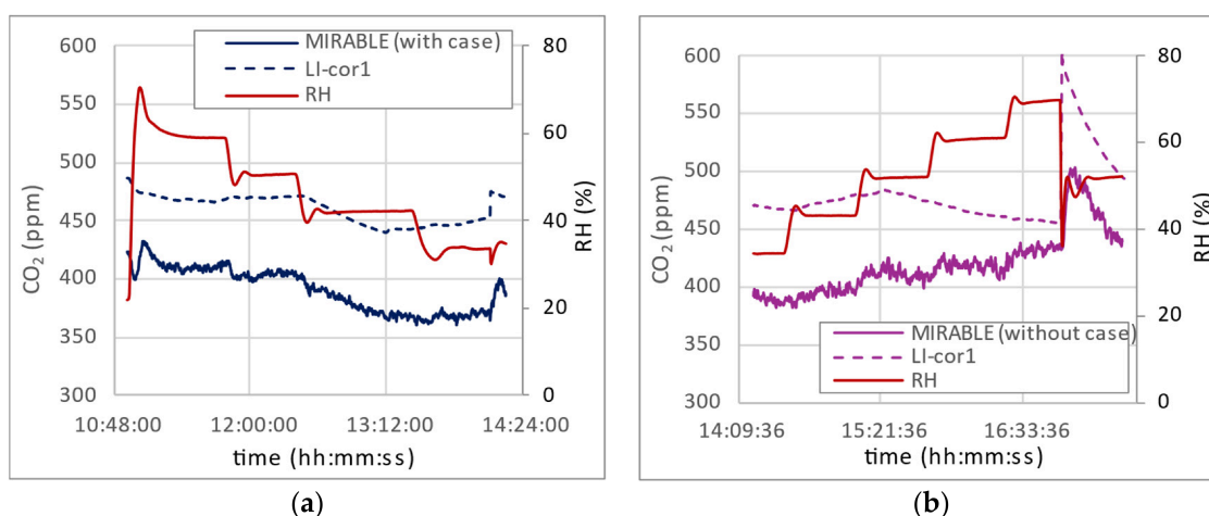
Figure 8. Comparison between MIRABLE sensor and LI-cor1 as a function of relative humidity at T = 23 °C: (a) with-case; (b) without-case.
