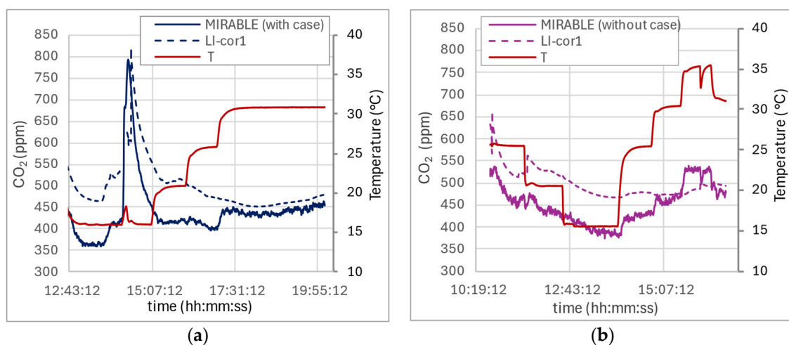
Figure 7. Comparison between MIRABLE sensor and LI-cor1 as a function of chamber temperature at constant relative humidity (50 %rh): (a) with-case; (b) without-case.
