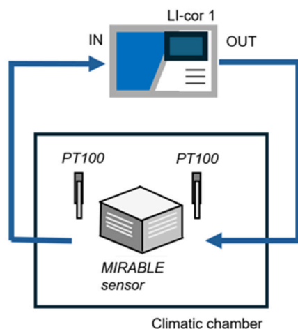
Figure 2. Scheme of the experimental set-up for the analysis of environmental influence factors on low-cost \text{CO}_2 sensor.
