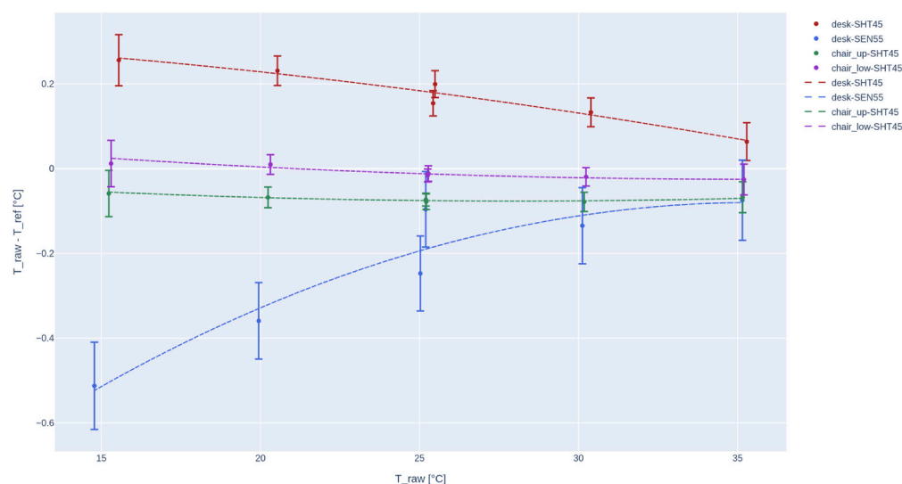
Figure 4. Measurement errors of all sensors with associated uncertainty bars ( k = 2 ) as a function of temperature, without the external case. Dashed lines represent second-order polynomial correction curves.
