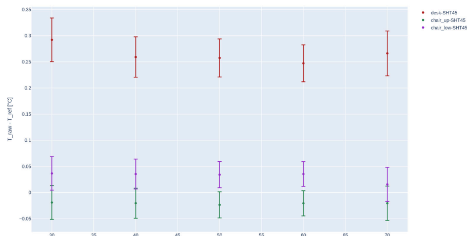
Figure 6. Measurement errors of SHT45 sensors as a function of relative humidity (without external case), at constant temperature T = 23 °C ( k = 2 ).
