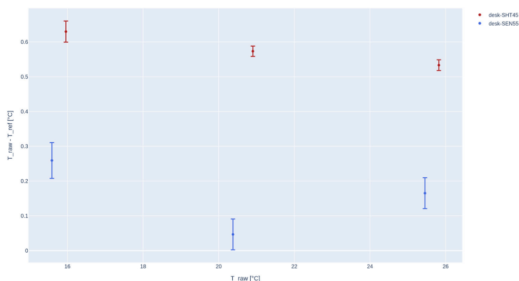
Figure 5. Measurement errors of desk-SHT45 and desk-SEN55 sensors with associated uncertainty bars ( k = 2 ) as a function of temperature, with the external case.
