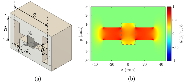
Fig. 3. (a) DEB-RW, the black block corresponds to the sample to be measured. (b) Real part of the E-field at the cross section z = 0 , at 2.5 GHz, the dashed outline shows the position of the sample. The dimensions in mm are: a = 90, b = 60, w = 18, h = 14 .
