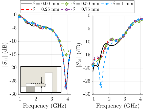
Fig. 4. Scattering parameters of the DEB-RW loaded with a small sample for different gap sizes \delta .
