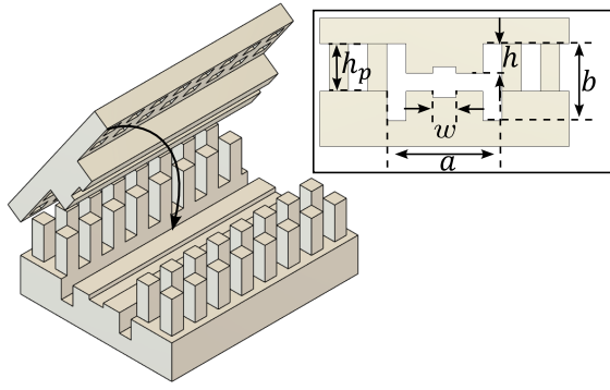
Fig. 7. Schematic of the gap waveguide implementation of the proposed DEB-RW. The dimensions in mm are: a = 90 , b = 60 , w = 18 , h = 14 , and h_p = 46 .
