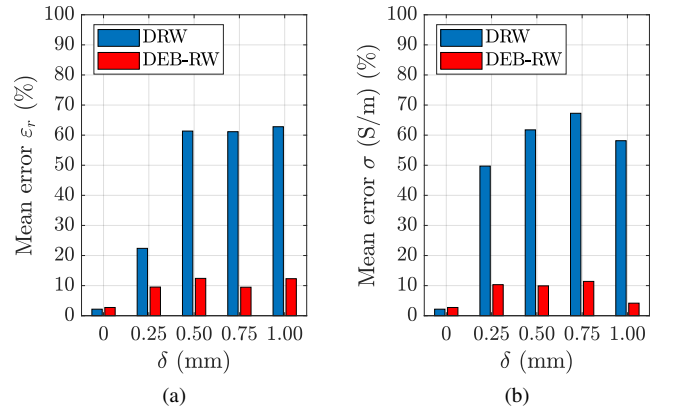
Fig. 6. Comparison of the relative error in the DPs retrieved from the D-RW and DEB-RW configurations: (a) relative permittivity, (b) conductivity.
