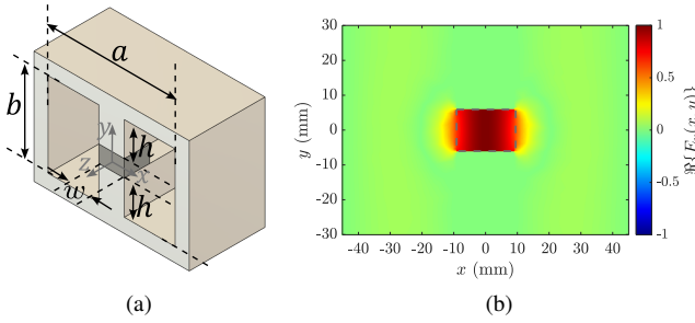
Fig. 1. (a) D-RW, the black block corresponds to the sample to be measured. (b) Real part of the E-field at the cross section z = 0 , at 2.5 GHz, the dashed outline shows the position of the sample. The dimensions in mm are: a = 90, b = 60, w = 18, h = 23 .
