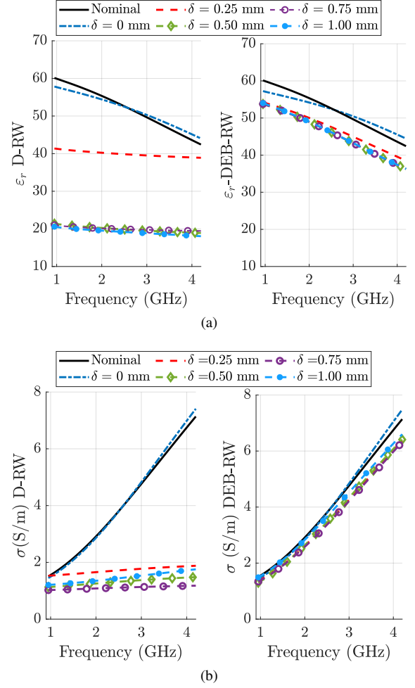
Fig. 5. DPs retrieved from the D-RW and DEB-RW. The first row shows the relative permittivity, and the second row shows the conductivity.
