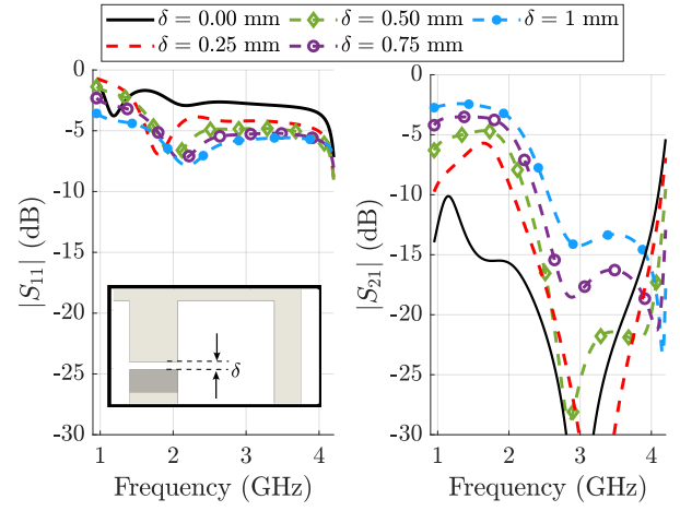
Fig. 2. Scattering parameters of the D-RW loaded with a small sample for different gap sizes \delta .
