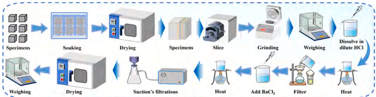
Fig. 6. Flow chart of the SO_4^{2-} PD test procedure.
