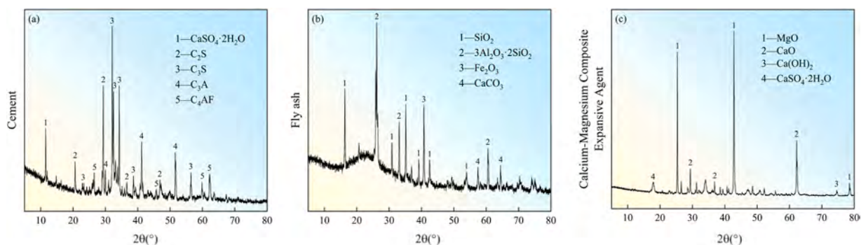
Fig. 1. Phase compositions of OPC, FA, and CMEA.
