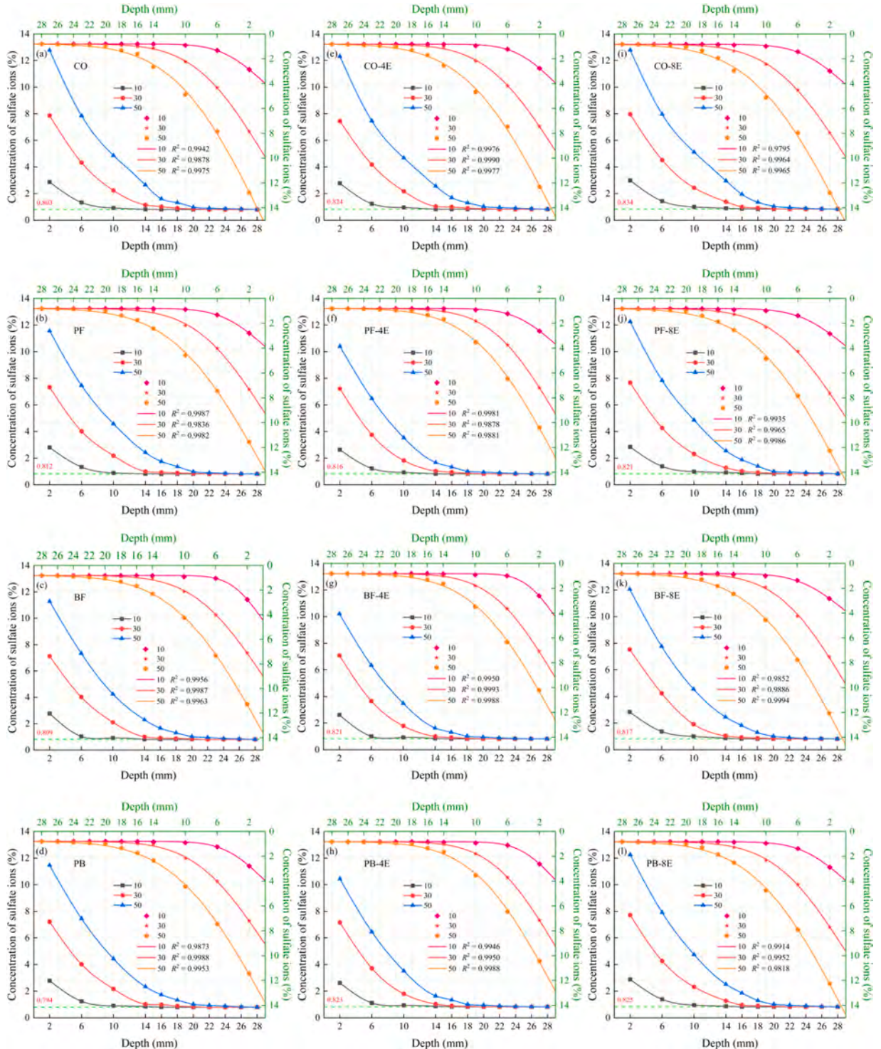
Fig. 10. Evolution of \text{SO}_4^{2-} concentration profiles in different specimens under sulfate DWs.
