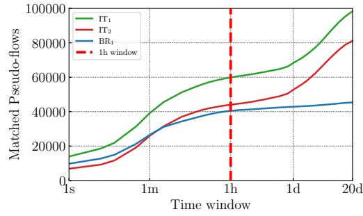
Figure 5: Follow-ups to UDP Replies: Sensitivity analysis of the time windows. The plot reports the number of matched pseudo-flows between the darknet and the RT-UDP subnet across the three deployments as the observation window expands from seconds to the full 20-day period.
