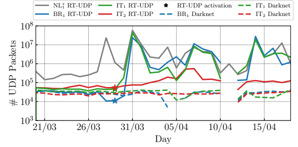
Figure 1: Daily packet counts before and after replying to UDP traffic. Each ★ marks an RT-UDP activation. A short outage is visible in some sensors.
