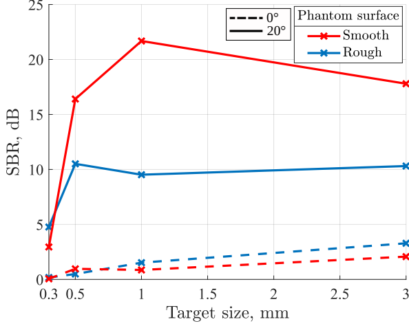
Fig. 14. Signal-to-background ratio versus target size for smooth and rough surface phantoms under normal ( 0^\circ ) and oblique ( 20^\circ ) incidence.
