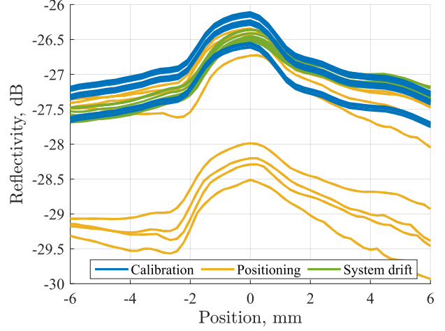
Fig. 15. Lateral reflectivity profiles at the air–phantom interface as a function of lateral position over a 12 mm scan across the target, with measurements grouped according to the investigated uncertainty contributions: calibration (blue), positioning (yellow), and system drift (green).
