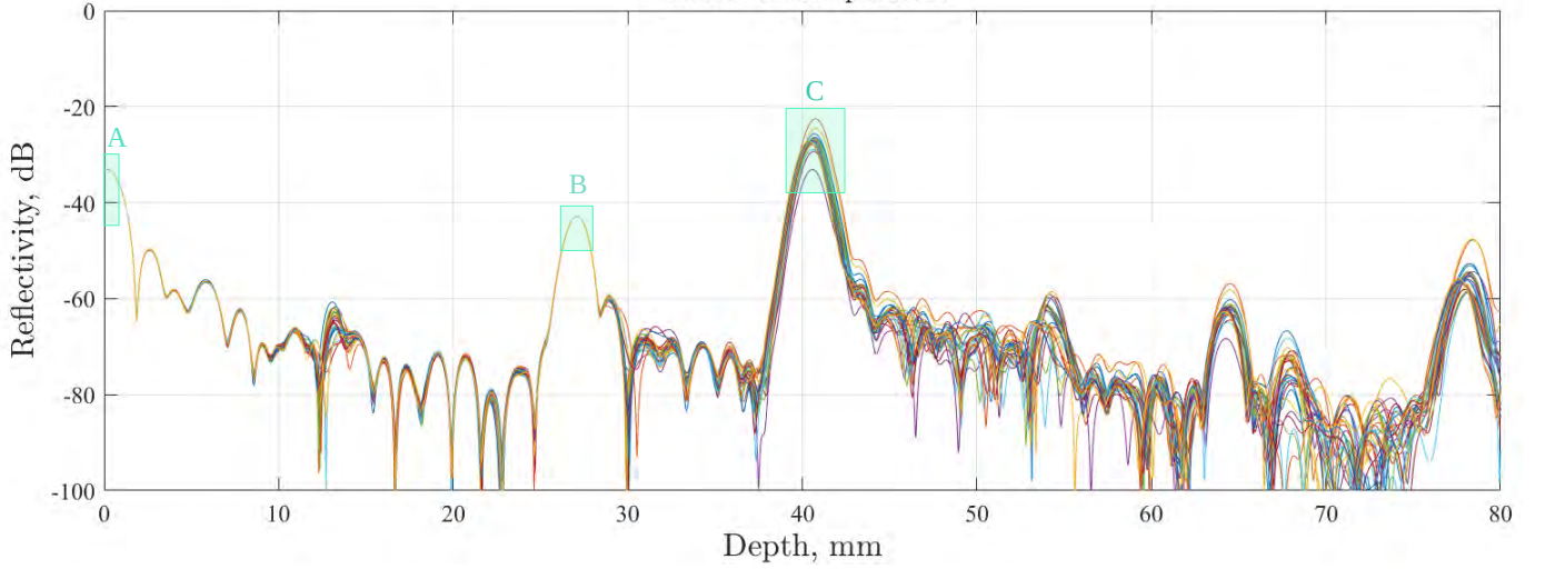
Fig. 10. Axial reflectivity profiles highlighting the calibration plane (A), antenna–air interface (B), and air–phantom interface (C), with each color corresponding to a distinct point along the scanning trajectory.
