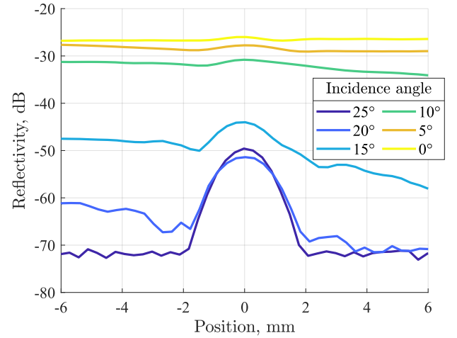
Fig. 11. Lateral reflectivity profiles at the air–phantom interface as a function of lateral position over a 12 mm scan across the target, centered at 0 mm, for different angles of incidence.
