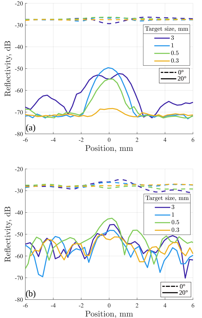
Fig. 13. Lateral reflectivity profiles at the air-phantom interface as a function of lateral position over a 12 mm scan across the target, centered at 0 mm, for phantoms with decreasing target size and different surface conditions: (a) smooth surface and (b) rough surface.
