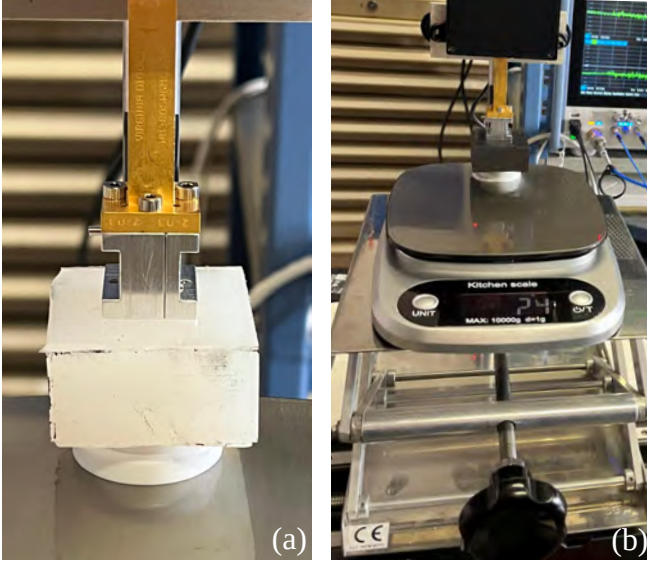
Fig. 3. Dielectric characterization of the silicone rubber samples. (a): close-up of an open-ended WR-1.5 waveguide in contact with the MUT; (b): measurement electronic scale on the elevation jack used to monitor the sample contact force.
