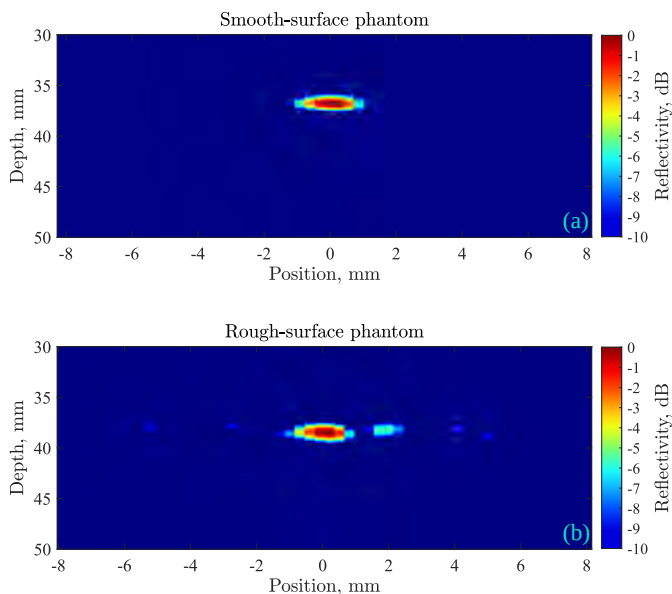
Fig. 16. B-scan images, obtained as a sequence of consecutive axial reflectivity profiles, of silicone rubber phantoms featuring a central target mimicking a skin lesion of 0.5 mm in size, surrounded by healthy skin, acquired with the contactless system at 20^\circ incidence. (a): smooth-surface phantom; (b): rough-surface phantom.
