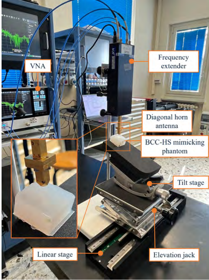
Fig. 9. Measurement setup for skin phantoms mimicking basal cell carcinoma comprising a VNA, the compact probe held vertically by a metal stand, the tilt stage, the elevation jack, and the high-precision linear stage. Close-up: the horn antenna scanning a phantom.
