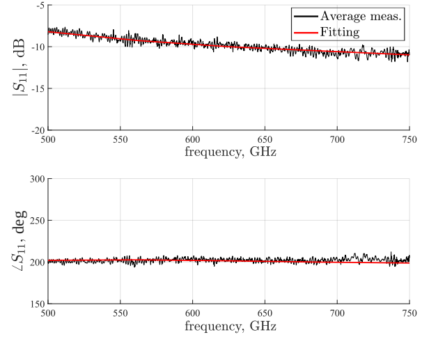
Fig. 5. Reflection coefficients averaged over applied pressure, measured with an open-ended waveguide in contact with a pure silicone rubber sample (black lines) and obtained from fitted full-wave simulations (red lines).
