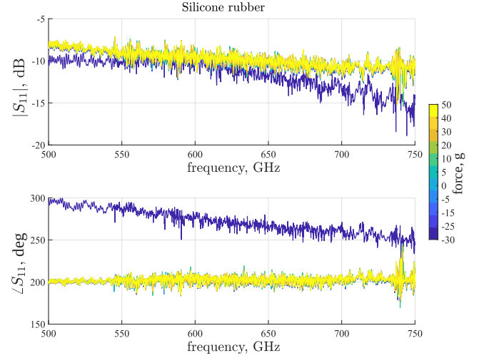
Fig. 4. Reflection coefficients of a pure silicone rubber sample at varying contact pressures with the open-ended waveguide; negative force values indicate persistent contact caused by the sample's adhesive behavior while lowering the laboratory jack, with detachment at -30 g.
