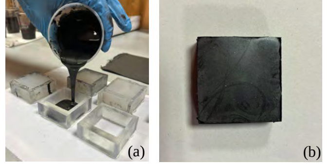
Fig. 2. The making of the silicone samples. (a): pouring of the silicone rubber and graphite mixture into the molds; (b): dried sample extracted from the mold (b).
