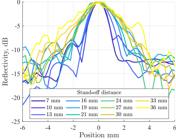
Fig. 12. Normalized lateral reflectivity profiles at the air-phantom interface for a 1 mm target, as a function of lateral position for different stand-off distances between the horn aperture and the phantom surface.
