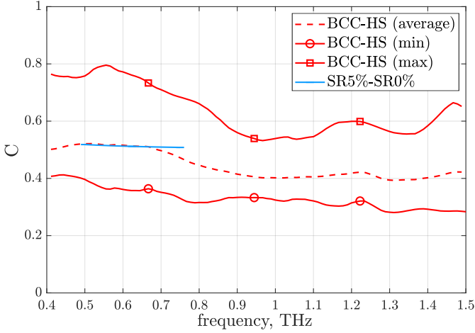
Fig. 1. Dielectric contrast between basal cell carcinoma (BCC) and healthy skin (HS), indicated in red, and between 5% and 0% graphite-loaded silicone rubber (SR), indicated in cyan.
