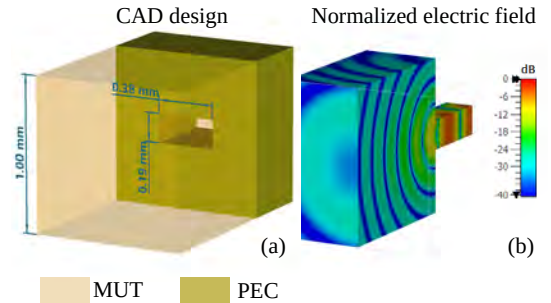
Fig. 6. Numerical model used for parametric full-wave simulations. (a): CAD design; (b): normalized electric field distribution.
