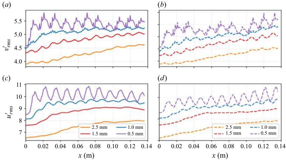
Figure 16. The r.m.s. of the wall-normal (a,b) and streamwise (c,d) velocity fluctuations above the liner for an acoustic excitation at SPL = 145 dB and f = 1400 Hz. (a,c) Upstream source. (b,d) Downstream source.
