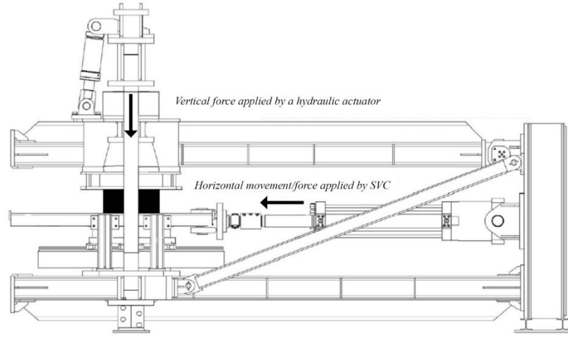
Figure 12 Testing machine
