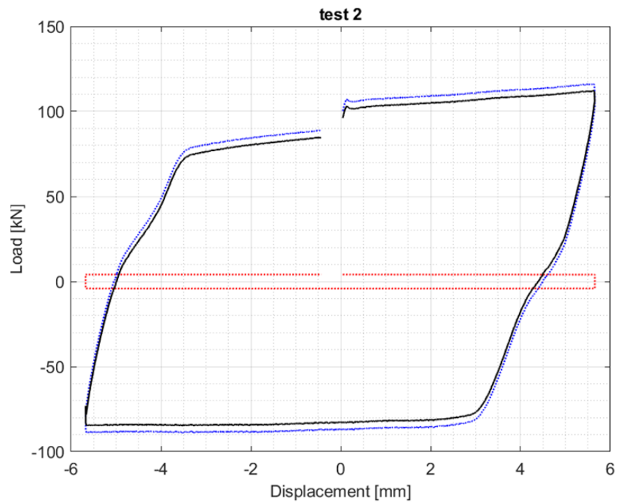
Figure 22 Semistatic test – multidirectional bearing – N = 2000 kN
