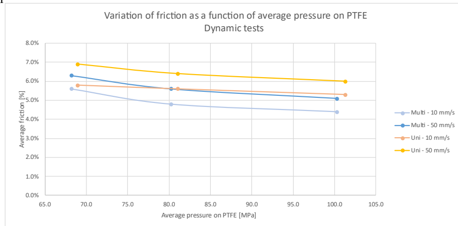
Figure 18 Variation of friction as a function of average pressure on PTFE in dynamic tests
