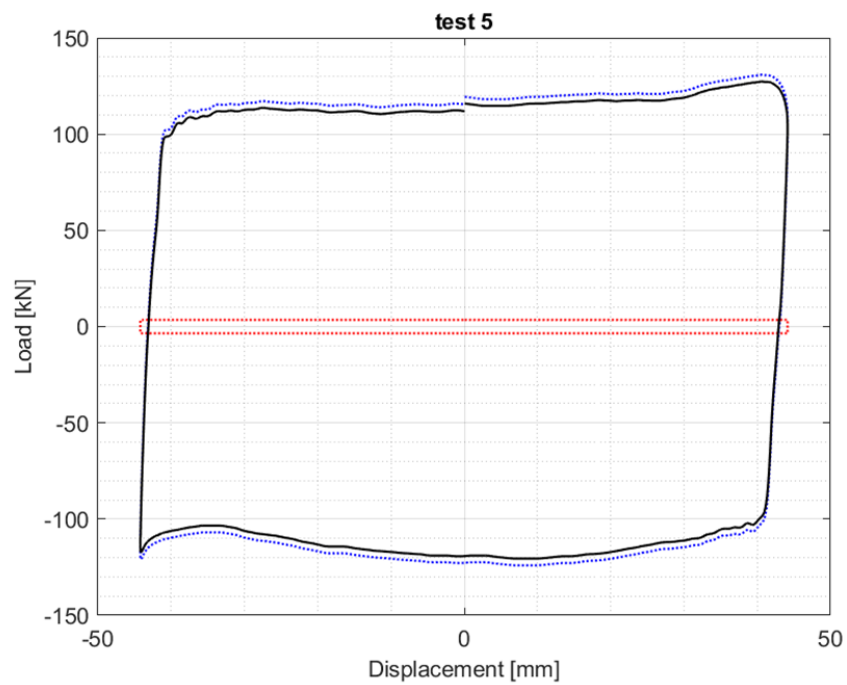
Figure 34 Dynamic test – unidirectional bearing – N = 1700 kN, v = 50 mm/s
