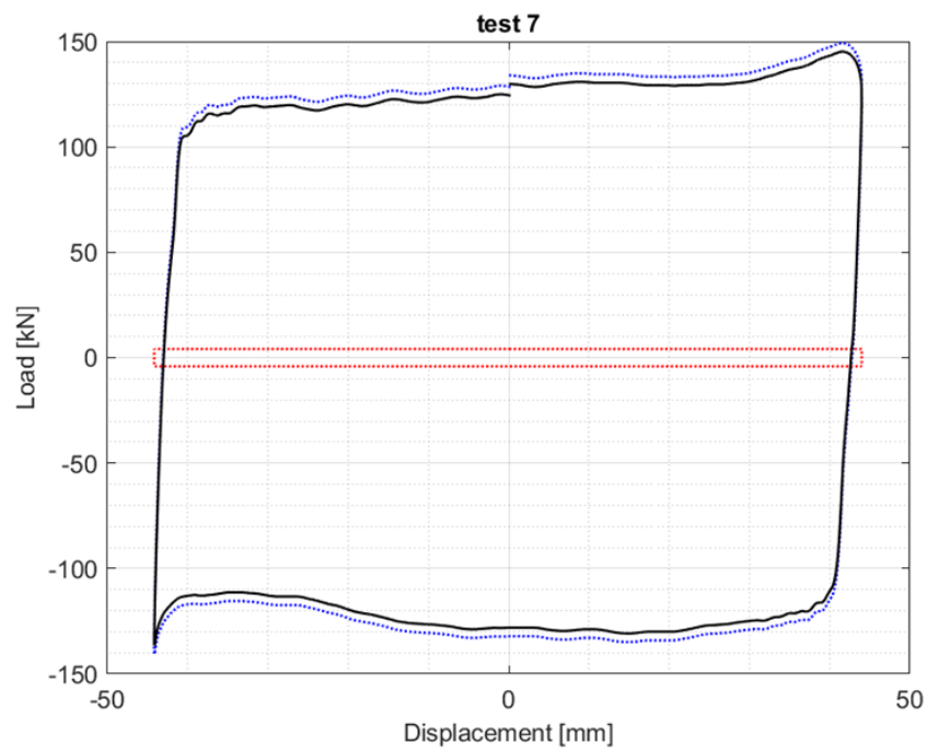
Figure 36 Dynamic test – unidirectional bearing – N = 2000 kN, v = 50 mm/s
