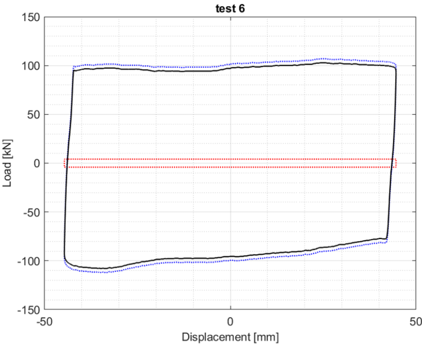
Figure 29 Dynamic test – multidirectional bearing – N = 2000 kN, v = 10 mm/s
