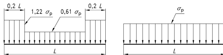
Figure 15 Alternative PTFE pressure distributions – extracted from EN-1337-2
