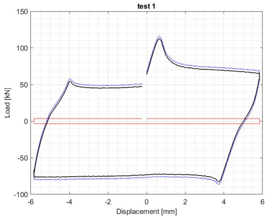
Figure 24 Semistatic test – unidirectional bearing – N = 1700 kN
