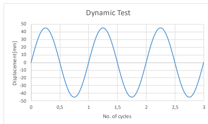
Figure 14 Cycles of displacements imposed on bearings for dynamic tests
