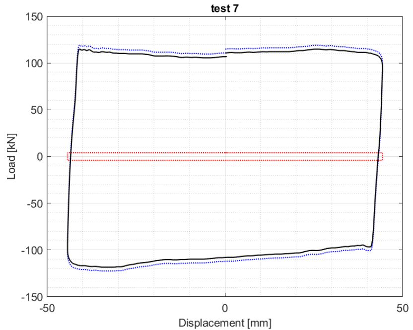
Figure 30 Dynamic test – multidirectional bearing – N = 2000 kN, v = 50 mm/s
