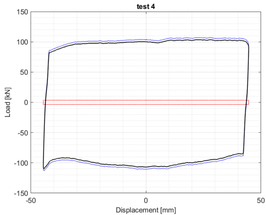
Figure 33 Dynamic test – unidirectional bearing – N = 1700 kN, v = 10 mm/s
