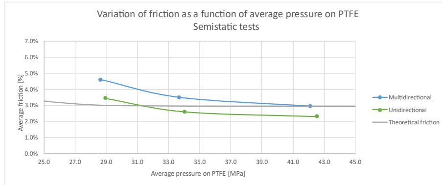
Figure 16 Variation of friction as a function of average pressure on PTFE
