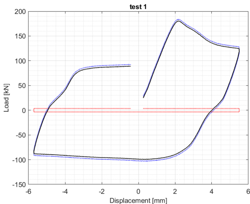
Figure 21 Semistatic test – multidirectional bearing – N = 1700 kN
