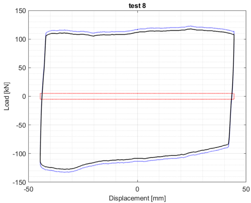
Figure 31 Dynamic test – multidirectional bearing – N = 2500 kN, v = 10 mm/s
