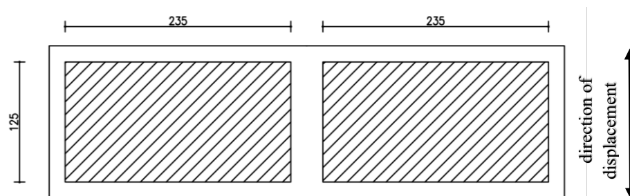
Figure 8 PTFE pads dimensions (in mm) - Unidirectional bearings
