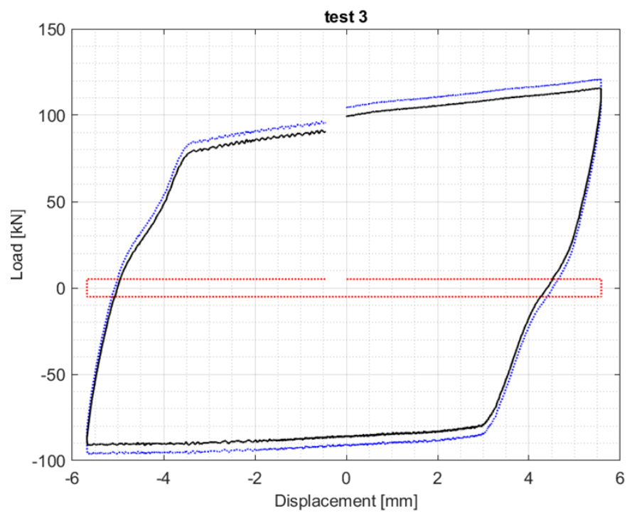
Figure 23 Semistatic test – multidirectional bearing – N = 2500 kN
