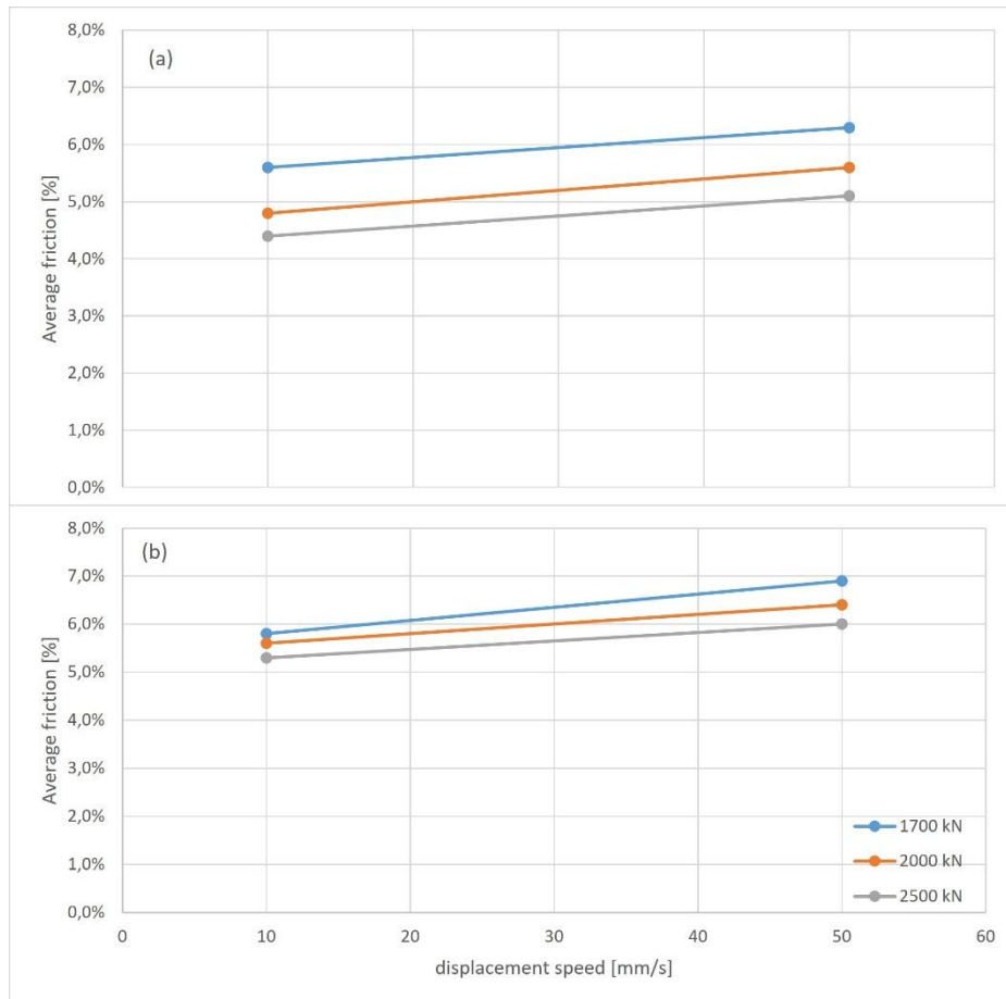
Figure 17 Variation of friction as a function of displacement speed (for multiple applied vertical loads) – (a) Multidirectional and (b) Unidirectional bearings
