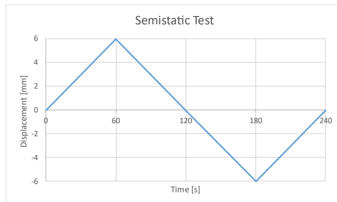
Figure 13 Displacement imposed over time on bearings for semi-static tests
