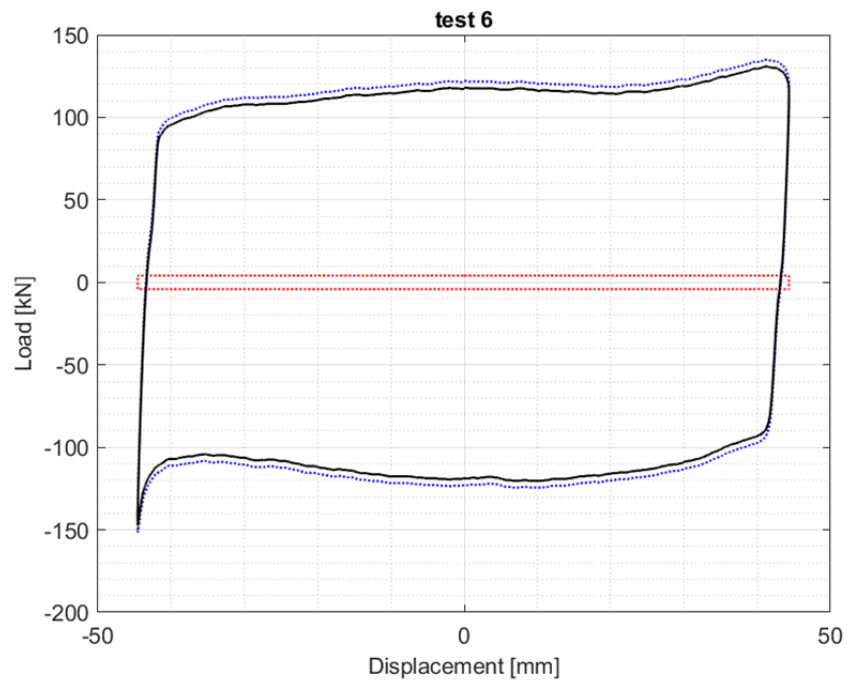
Figure 35 Dynamic test – unidirectional bearing – N = 2000 kN, v = 10 mm/s
