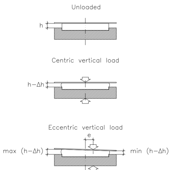
Figure 3 Deformation of PTFE in a sliding support - adapted from “Apparecchi d’appoggio” (Marioni, 1983)
