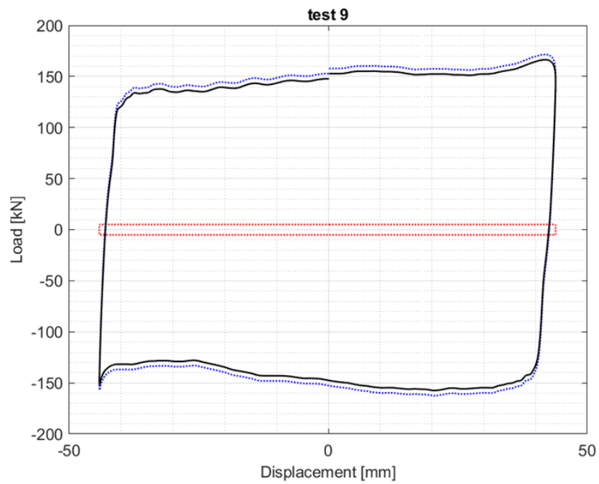
Figure 38 Dynamic test – unidirectional bearing – N = 2500 kN, v = 50 mm/s
