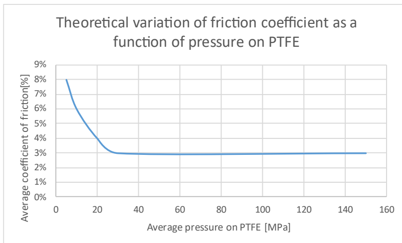
Figure 2 Theoretical variation of friction coefficient as a function of pressure on PTFE
