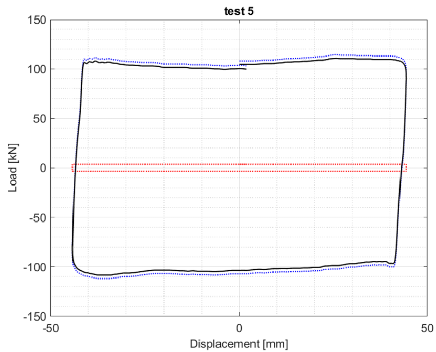
Figure 28 Dynamic test – multidirectional bearing – N = 1700 kN, v = 50 mm/s
