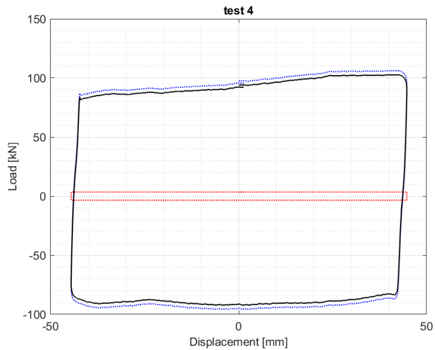
Figure 27 Dynamic test – multidirectional bearing – N = 1700 kN, v = 10 mm/s
