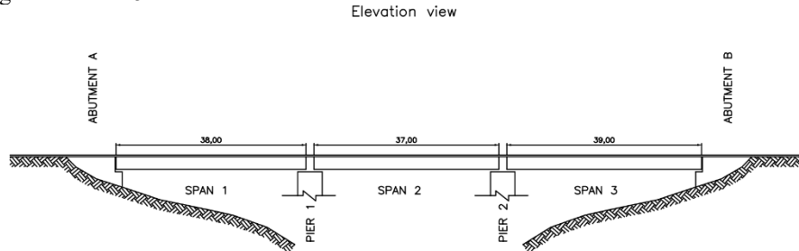
Figure 4 Bridge elevation view
