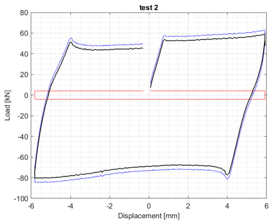
Figure 25 Semistatic test – unidirectional bearing – N = 2000 kN
