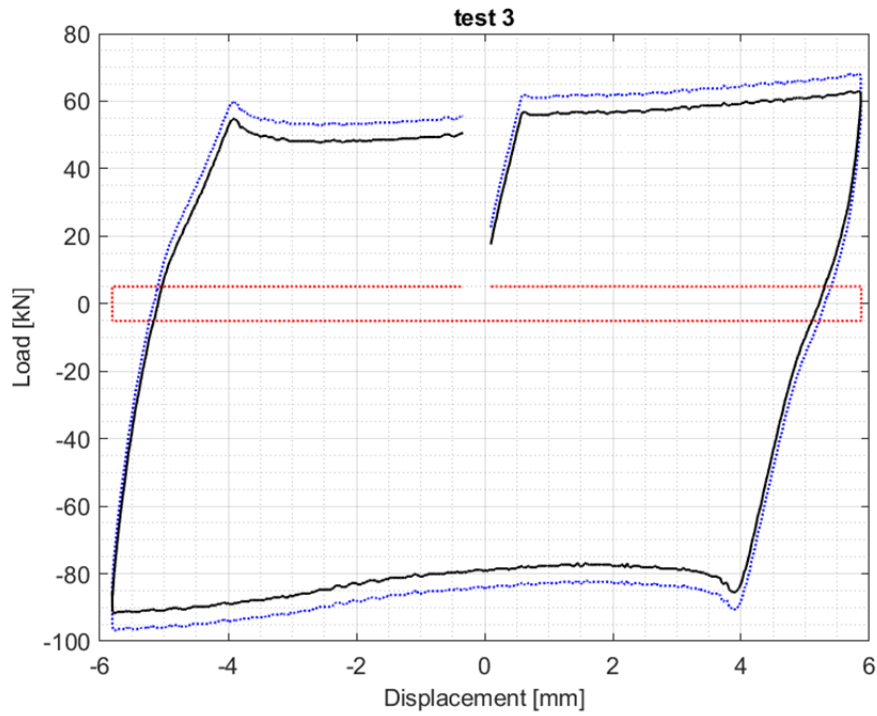
Figure 26 Semistatic test – unidirectional bearing – N = 2500 kN
