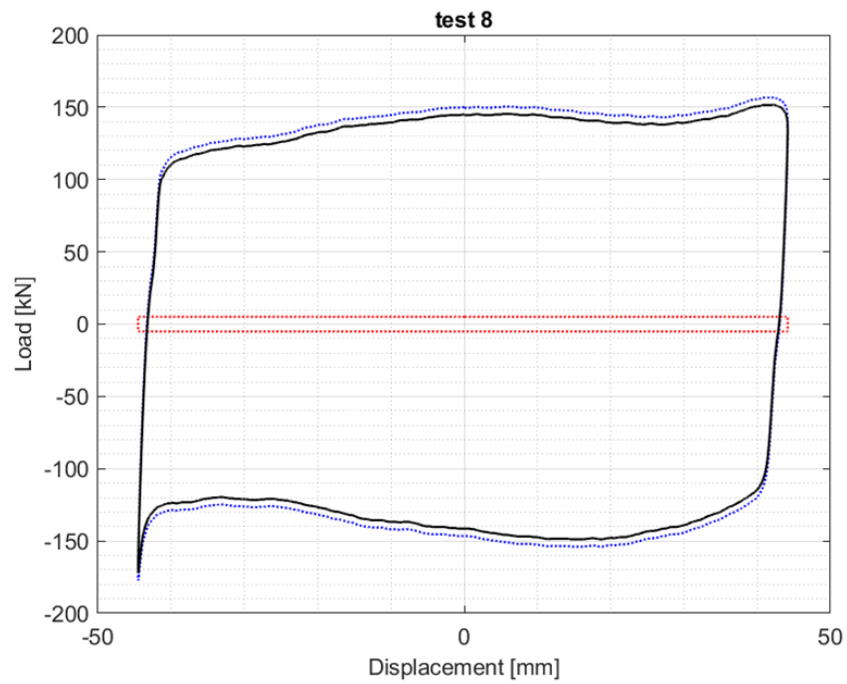
Figure 37 Dynamic test – unidirectional bearing – N = 2500 kN, v = 10 mm/s
