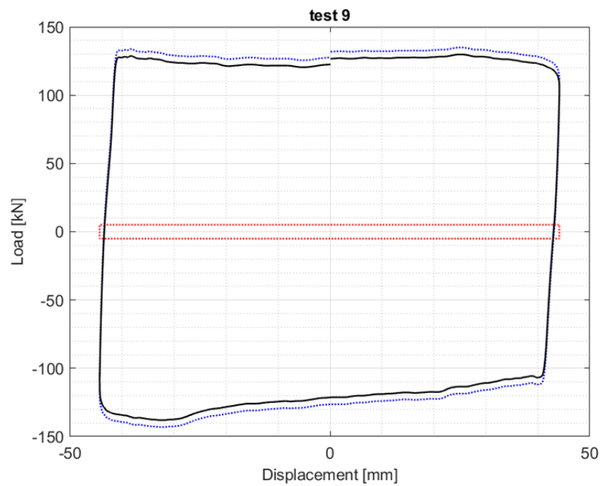
Figure 32 Dynamic test – multidirectional bearing – N = 2500 kN, v = 50 mm/s
