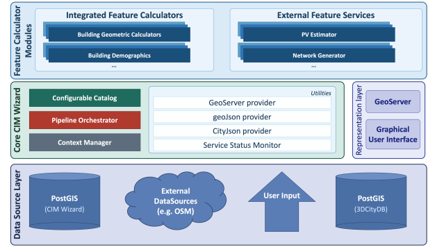
Fig. 2. High-level architecture schema
