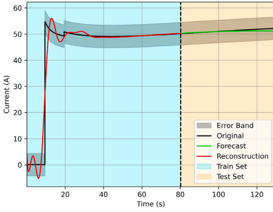
Fig. 16. Reconstruction and forecast of the beam current for rank r = 9 and train cutoff 0.62.
