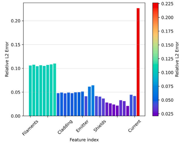
Fig. 9. Relative L_2 error per feature considering optimum rank r = 12 .
