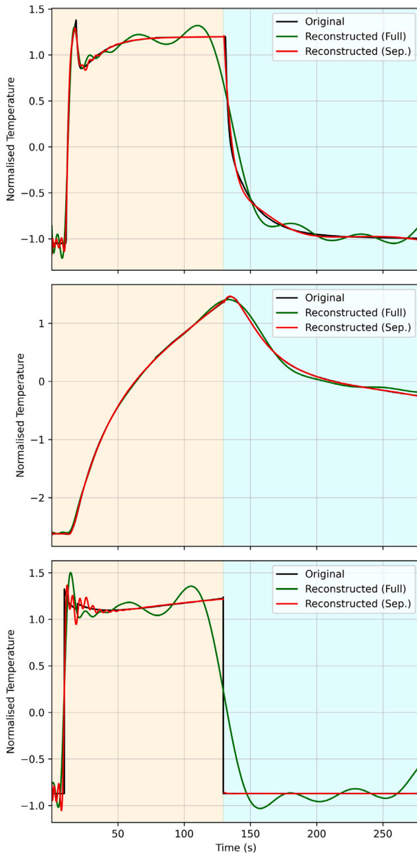
Fig. 10. Feature reconstruction for the filament, emitter and beam current for the case in which a single surrogate model accounts for the entire time range (green) and the case in which on-phase and off-phase are separated, and two independent surrogate models are built. All models have rank r = 12 .
