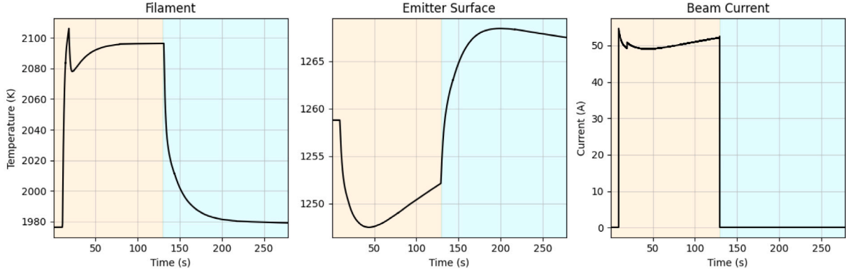
Fig. 3. Temporal behaviour of all quantities of interest of the MIG lumped model. The dataset includes both the on-phase (orange background, up to t_1 = 129 s) and the off-phase (cyan background). The different time scales of the different features, as well as the different dynamics of the two phases, can be clearly seen.
