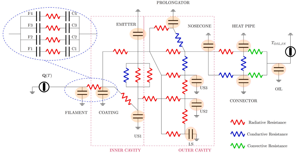
Fig. 2. Equivalent electrical circuit of the heat transfer between the various bodies in the MIG. Components are highlighted in orange. All components within a cavity exchange heat through radiation with all components within the same cavity. Resistances shown here are just for visualization purposes, to highlight the different heat transfer mechanisms between different components of the MIG.
