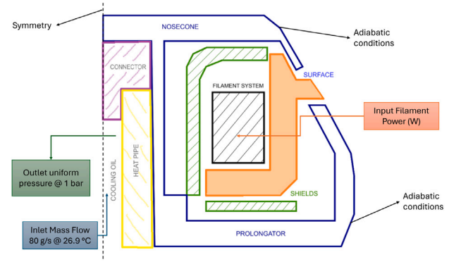
Fig. 1. Schematic representation of the MIG cathode (modified from [3]), along with the relevant boundary conditions. Upper and lower shields are shown in dashed green, while the emitter is marked in orange. The oil flows from the bottom of the central pipe upward to the connector (purple, dashed), then it descends downwards in contact with the heat pipe (yellow, dashed). The MIG cathode is vacuum-sealed. The figure is not to scale.
