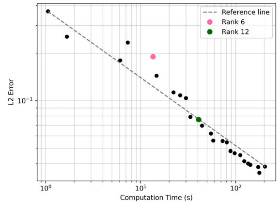
Fig. 8. Pareto front of the multi-objective optimization problem of the selection of the optimal rank, comparing computational times (x-axis) and overall relative L_2 error (y-axis). Both knee value (pink) and optimum rank (green) are reported as well, with respect to the reference line.
