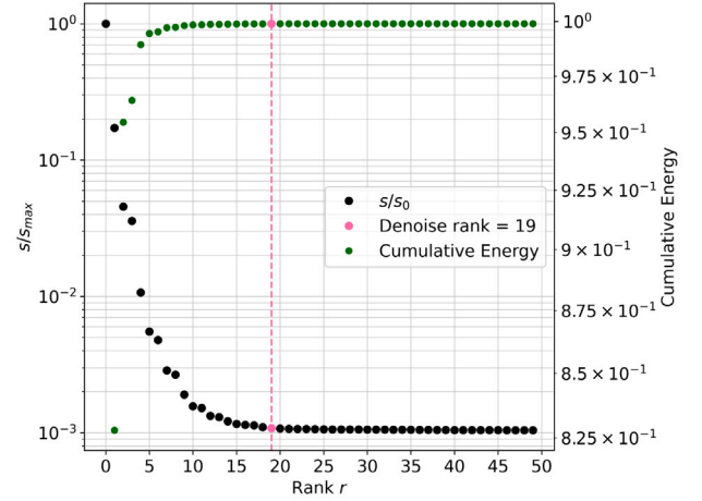
Fig. 6. Singular values of the embedded Hankel matrix (see Eq. (34)) (black) and cumulative energy (green). As a rule of thumb, the ‘elbow’ in the singular values separates physical from noisy features.
