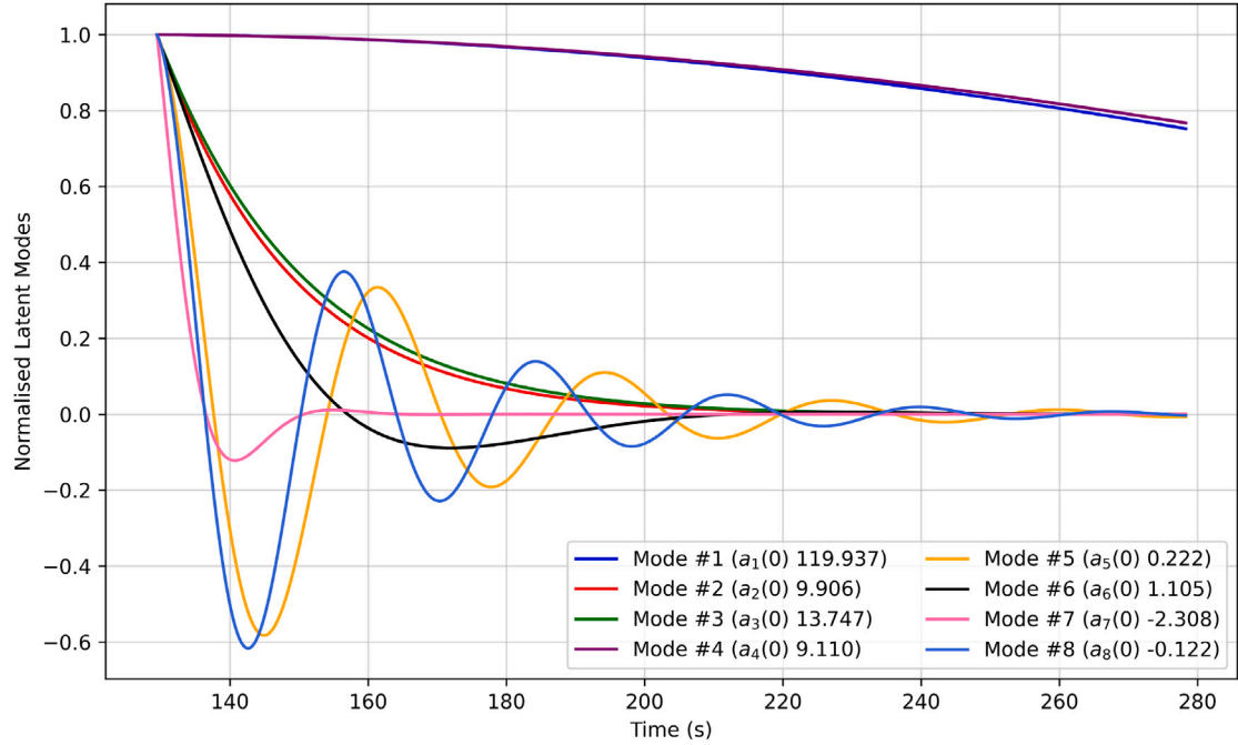
Fig. 12. First eight temporal modes for the off-phase, ranked according to the magnitude of the associated singular value.
