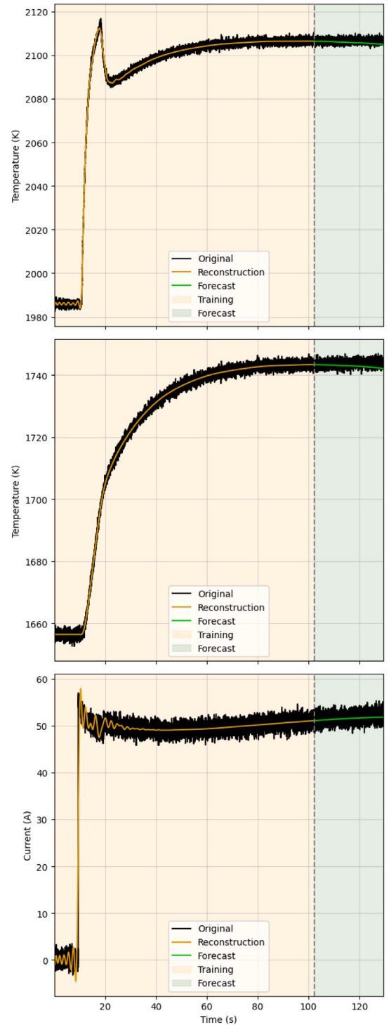
Fig. 15. Reconstructed (gold) and forecast (green) features (from top to bottom: filament, cladding, beam current) for the case r = 24 and cutoff training value 79%.
