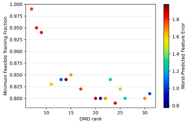
Fig. 14. Minimum allowed cutoff training value for different ranks, under constraint (30) for all features of interest. The maximum absolute error is reported as well.
