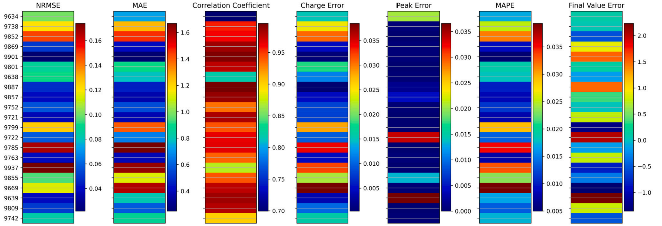
Fig. 4. Validation summary for the considered pulses (on-phase), using the following metrics: NRMSE, MAE, correlation coefficient, charge error, peak error, MAPE, absolute difference at the last time step.
