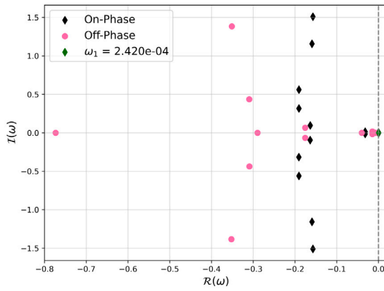
Fig. 13. Eigenvalues of the surrogate matrix \tilde{A} , considering separately the on-phase (black) and the off-phase (pink). The magnitude of the least stable mode is reported in green.
