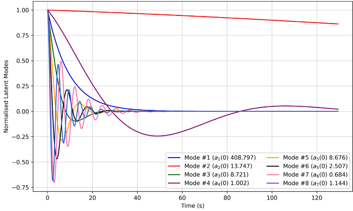
Fig. 11. First eight temporal modes for the on-phase, ranked according to the magnitude of the associated singular value.
