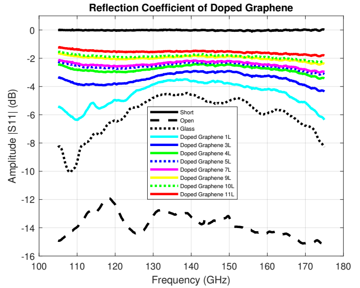
Fig. 3. Measured results of doped graphene samples in the 110-170 GHz frequency band.
