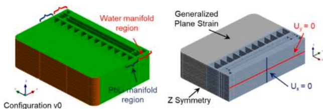
Fig. 22. Mechanical restraints.
