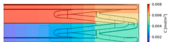
Fig. 15. Steady-state tritium concentration inside PbLi.
