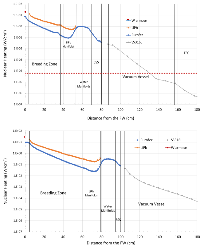
Fig. 5. Inboard (upper panel) and outboard (lower panel) nuclear heating density radial profiles. The red dotted line refers to the design target for the heat load on the TFC ( 5 \cdot 10^{-5} W/cm 3 ).
