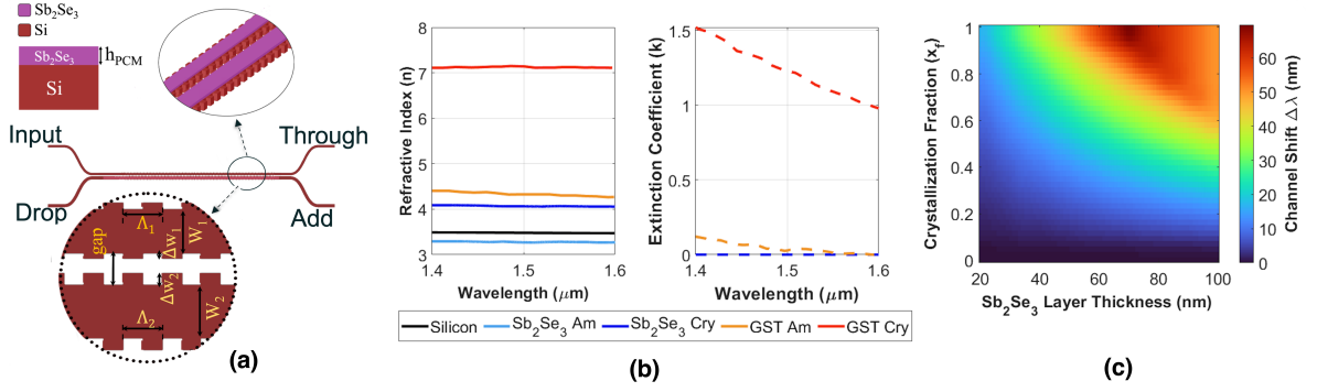
Fig. 1: (a) Schematic of the GACDC structure under investigation. (b) Refractive index and extinction coefficient for \text{Sb}_2\text{Se}_3 and \text{Ge}_2\text{Sb}_2\text{Te}_5 . (c) Drop channel wavelength shift ( \Delta\lambda ) as a function of the crystallization fraction ( X_f ) and \text{Sb}_2\text{Se}_3 thickness.
