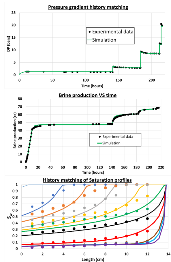
Fig. 9. Experimental and inversion results for the primary drainage unsteady state experiment.
