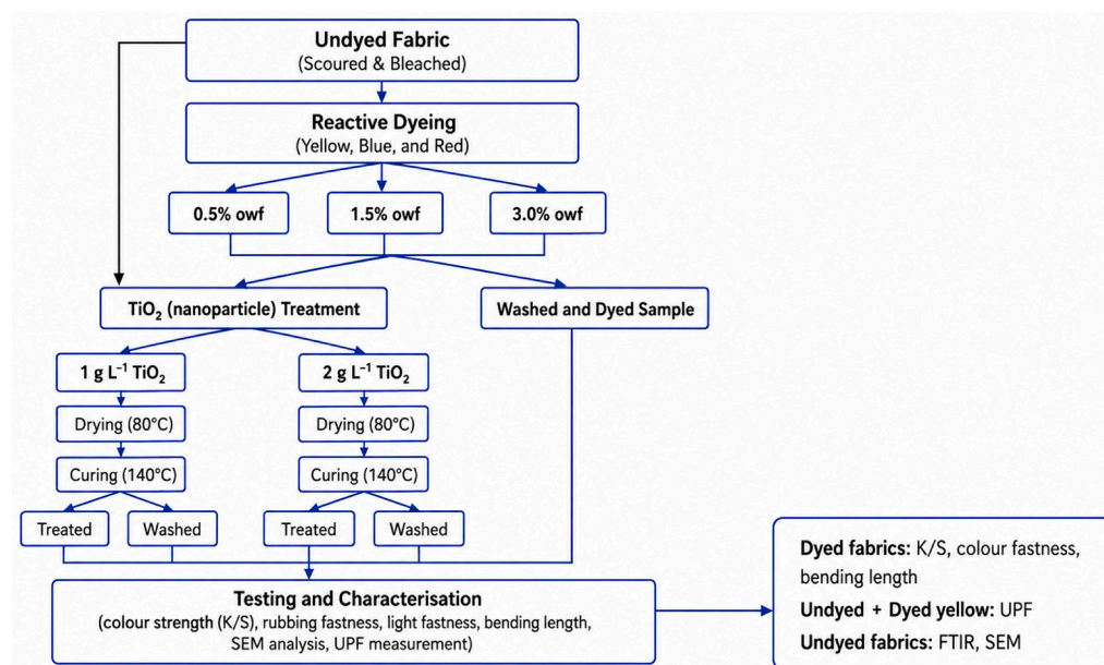
Figure 1. Schematic representation and sample preparation workflow. FTIR, SEM and UPF analyses were also performed on bleached \text{TiO}_2 -treated cotton.
