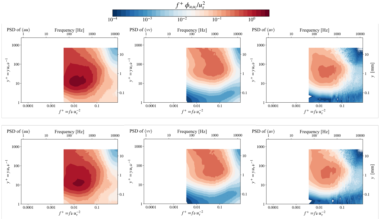
Figure 6. High-frequency uu (left column), vv (center column) and uv (right column) PSD distributions for the unforced flow (top row) and for the V_{pp} = 8 kV forced flow (bottom row) at \text{Re}_\tau = 14400 .
