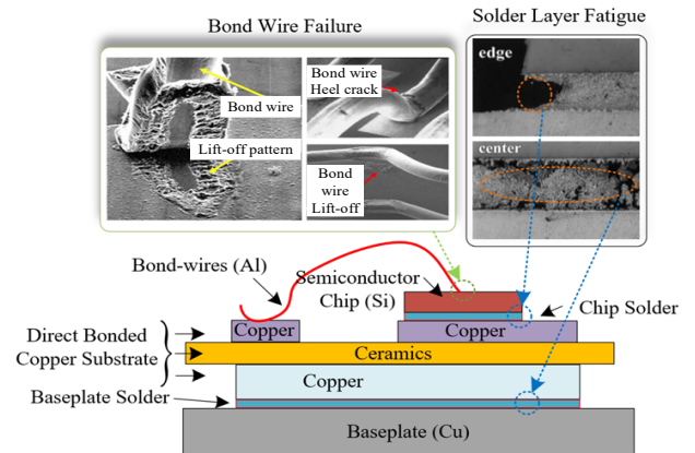
Fig. 1. Diagram of a standard IGBT module and its dominant package-related wear-out failure mechanisms [4].
