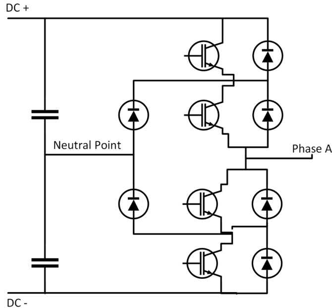
Fig. 10. One leg of the NPC inverter system of the Danfoss TLX PRO+ (the other two identical legs, the L-filter, and three parallel input boost converters are not pictured).
