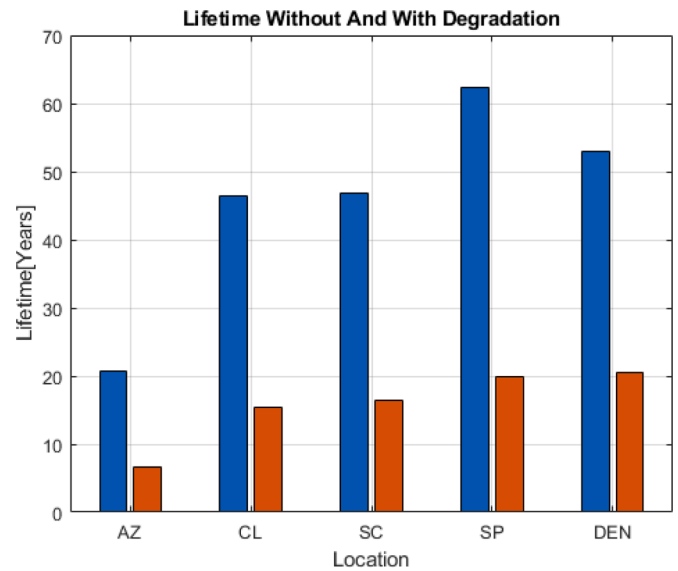
Fig. 14. Lifetime prediction without(blue) and with degradation(red) of Converter 2. (For interpretation of the references to colour in this figure legend, the reader is referred to the web version of this article.)
