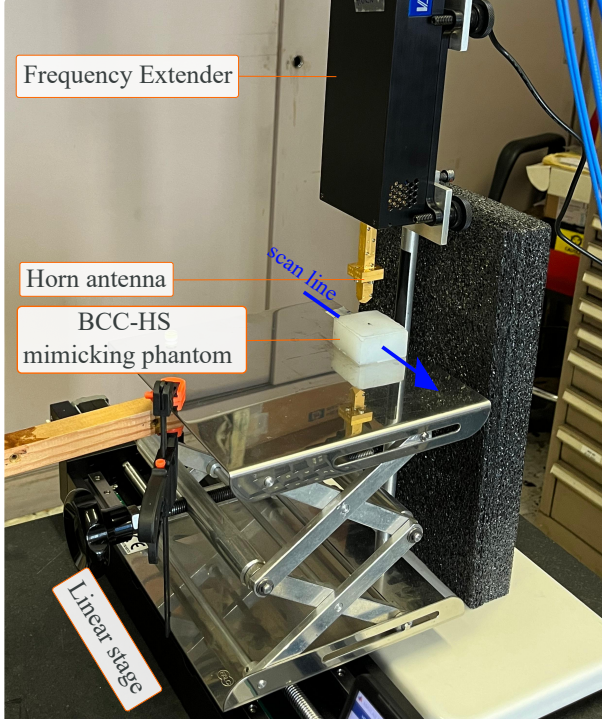
Fig. 1. Measurement setup close-up showing the compact probe mounted vertically on a metal stand, with the phantom supported by an elevation jack and positioned on a high-precision linear stage.
