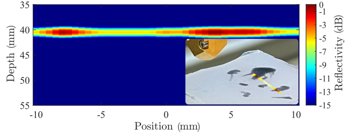
Fig. 2. B-scan image of a silicone rubber phantom featuring a BCC target pattern mimicking a skin lesion surrounded by healthy skin, acquired in the WR-1.5 frequency band.
