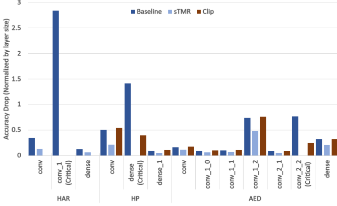
Fig. 2. Normalized accuracy drop per layer for the original, sTMR, and Clip versions of the HAR, HP, and AED models for the Stellar E board.
