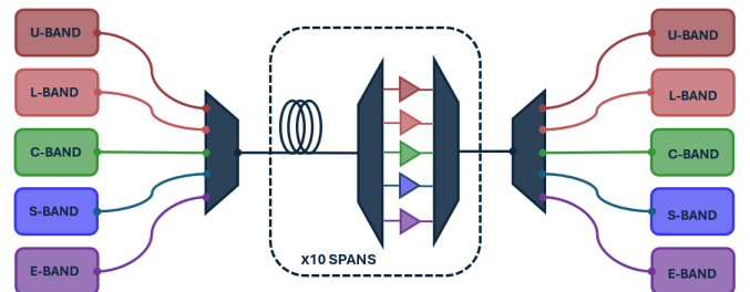
Fig. 1. Simulation setup.
