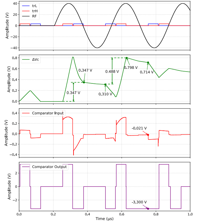
FIGURE 14. Example of constructive accumulation of \Delta V_C over multiple bit periods, showing the comparator input voltage eventually crossing the threshold and causing an error before the fourth bit.
