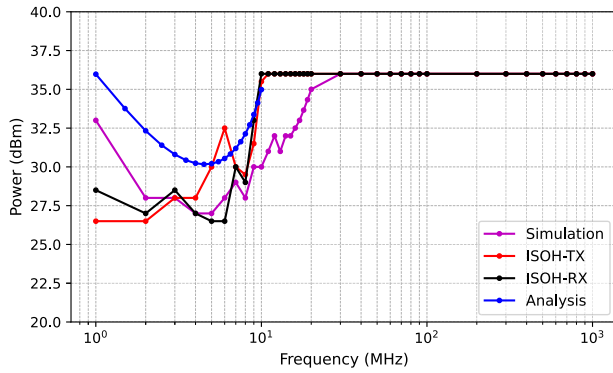
FIGURE 15. Susceptibility level of the VIF for analytical model, simulation, and measurement results.
