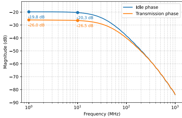
FIGURE 18. EMI to comparators' CM transfer function.
