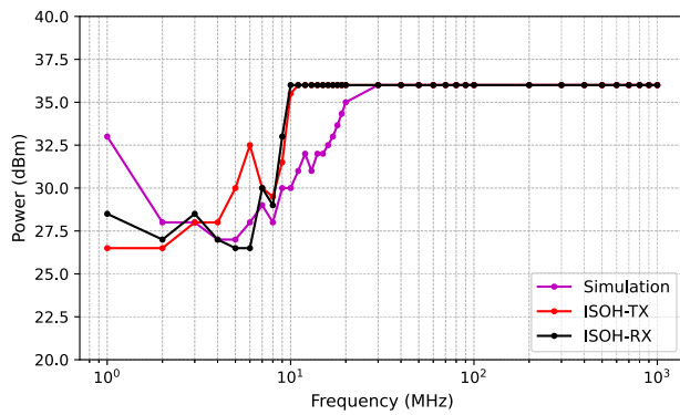
FIGURE 7. Comparison between the measured susceptibility levels of the VIF in transmitter (ISOH-TX) and receiver (ISOH-RX) modes, and the susceptibility level obtained from simulation.
