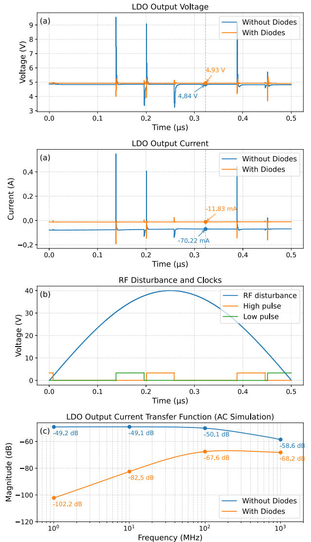
FIGURE 10. LDO regulator output simulations with and without diodes: a) the LDO regulator output current and voltage, b) 1 MHz RF signal along with clocks for a half positive period of the RF signal, c) Transfer function amplitude from EMI source to LDO regulator output current.
