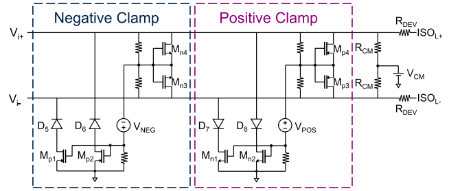
FIGURE 19. Simplified schematic of the clamp circuit.
