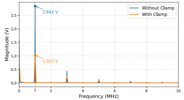
FIGURE 20. Common-mode FFT magnitude at comparator input with and without clamp circuits at 1 MHz RF disturbance.
