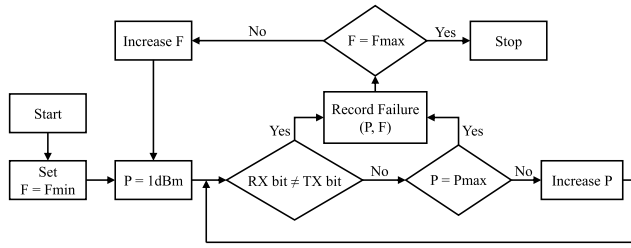
FIGURE 4. Flowchart of the DPI test procedure.
