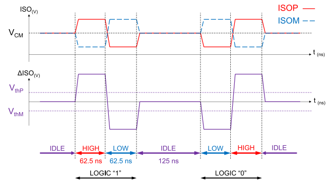
FIGURE 3. VIF protocol waveforms.
