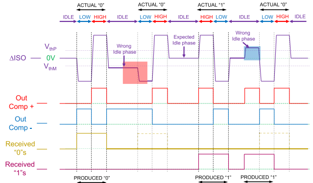
FIGURE 8. Different communication errors observed due to idle phase misbehavior.
