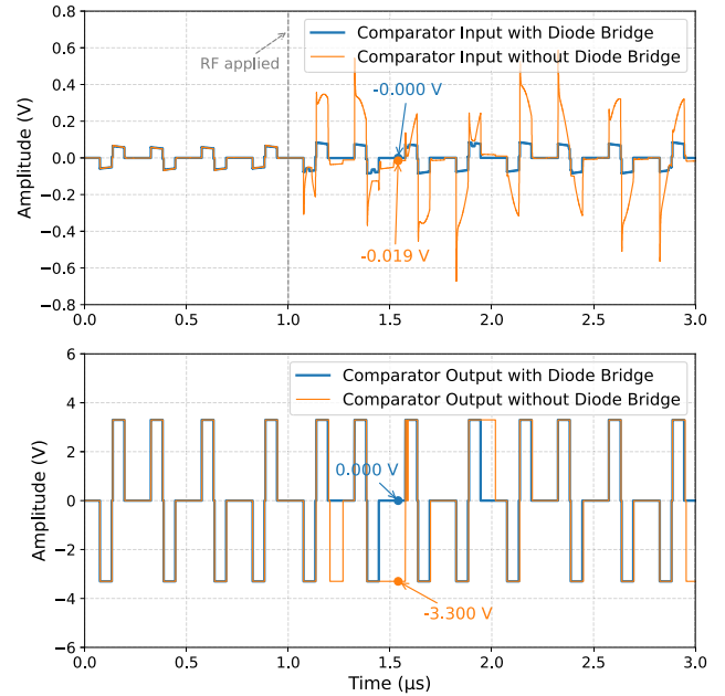
FIGURE 17. Comparison of comparator input and output waveforms with and without the diode bridge countermeasure under EMI excitation.
