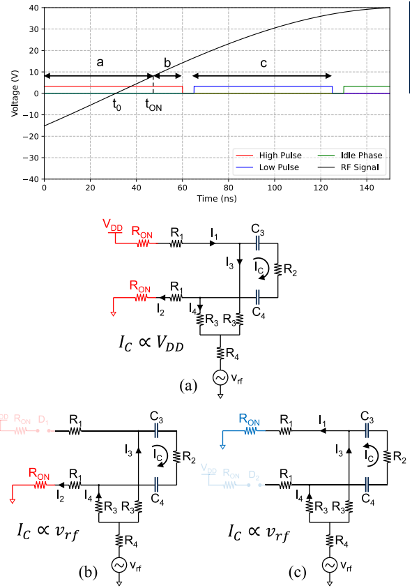
FIGURE 13. Time intervals and corresponding equivalent circuits for the worst-case failure scenario under EMI. The top plot shows the different time intervals (a, b, and c) created by a 2 MHz RF disturbance. The bottom diagrams show the equivalent circuit for each respective interval.
