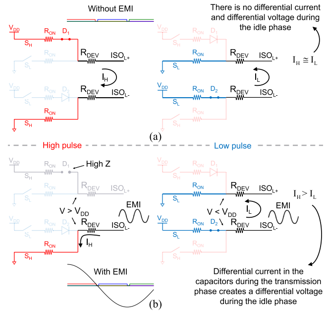
FIGURE 11. Pictorial representation of the failure mechanism: (a) Balanced currents during high and low pulses without EMI, leading to zero differential voltage; (b) when a sufficiently large common-mode EMI temporarily turns off one diode, the branch symmetry is broken, the capacitor currents become unequal, and the resulting unbalanced stored charge appears as a differential disturbance during the idle phase.
