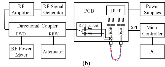
FIGURE 6. Experimental DPI test setup: (a) photograph of the laboratory bench and (b) functional block diagram of the measurement.
