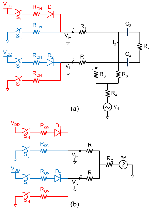
FIGURE 12. Simplified equivalent circuits used for analytical evaluation: a) initial model including C_3 and C_4 ; b) resistive model after simplification.
