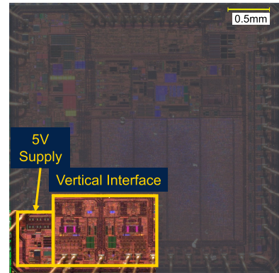
FIGURE 22. Die micrograph showing the VIF and 5V LDO supply area.
