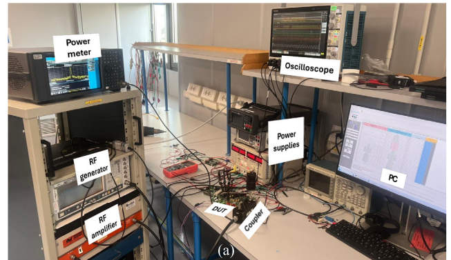
FIGURE 5. DPI test structure for the proposed VIF.
