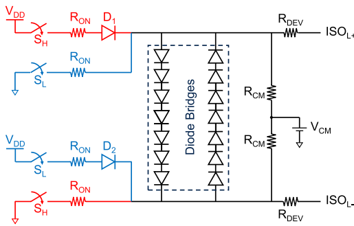
FIGURE 16. Schematic view of the diode strings to clamp the differential voltage.
