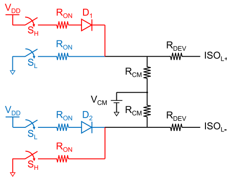
FIGURE 9. VIF structure with protective diodes.
