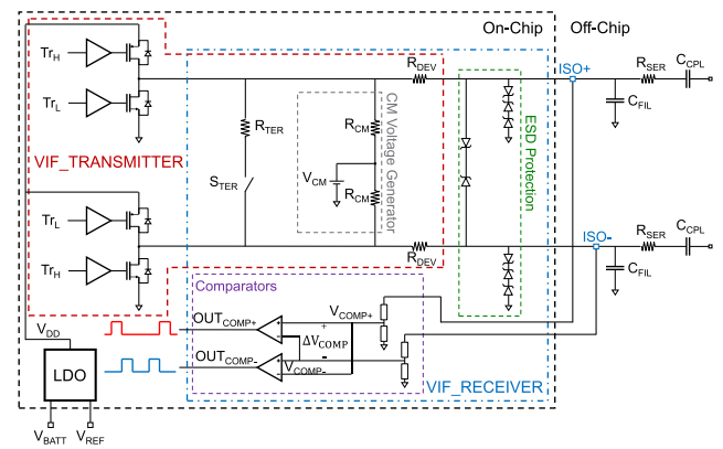
FIGURE 2. Schematic view of the VIF considered in this work.
