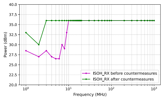
FIGURE 23. Measured susceptibility level of the VIF receiver (ISOH-RX) before and after implementing the proposed countermeasures.
