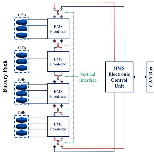
FIGURE 1. A typical BMS structure.
