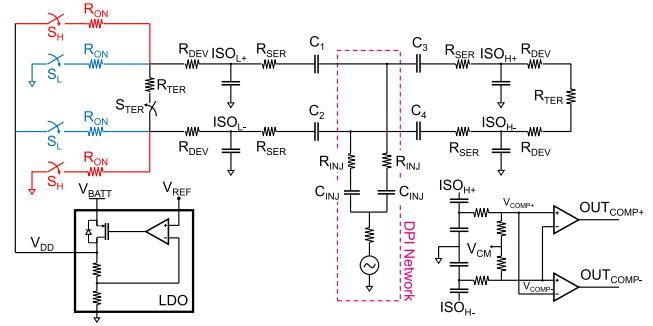
FIGURE 5. DPI test structure for the proposed VIF.
