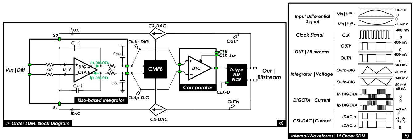
FIGURE 3. a) Sigma-Delta modulator block diagram, b) Waveforms of critical section of each block.
