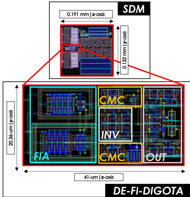
FIGURE 7. Chip layout view for the proposed modulator and fully differential FI-DIGOTA (DE-FI-DIGOTA).
