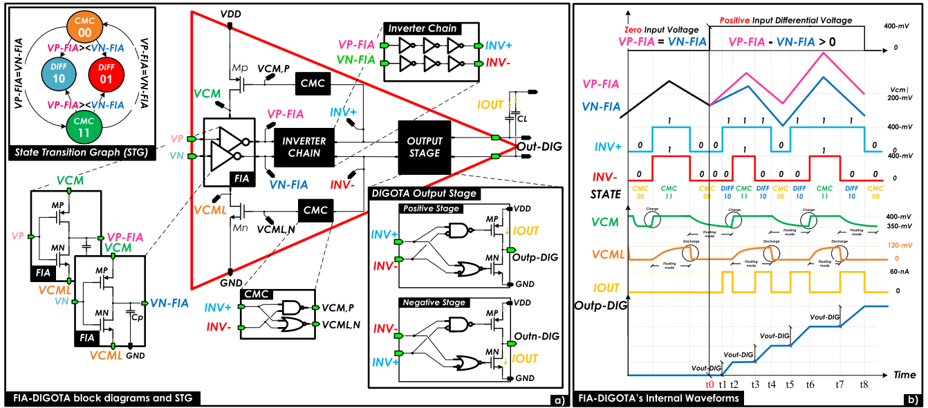
FIGURE 1. a) State-transition graph (STG) and FI-based DIGOTA block diagram, b) Waveforms of input/output of each block for zero and positive input differential voltage.
