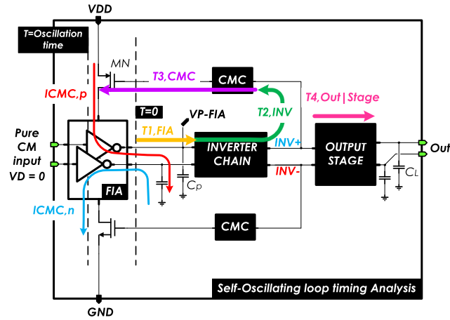
FIGURE 10. FI-DIGOTA self oscillation timing loop analysis under pure common-mode input condition.
