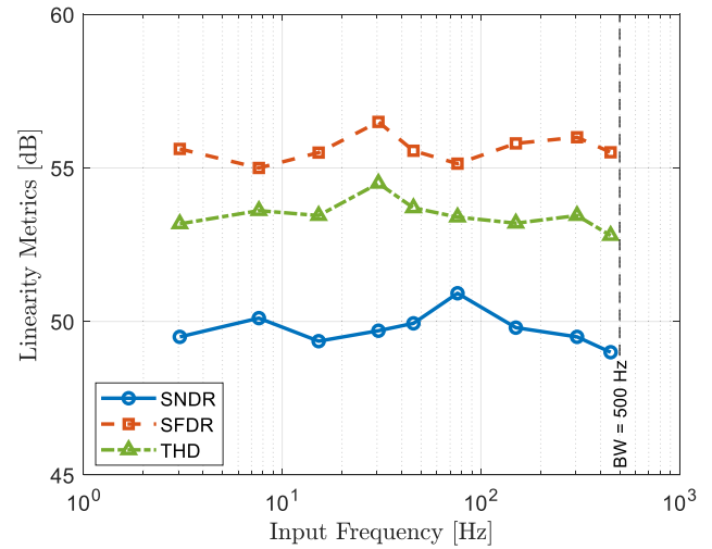
FIGURE 12. SNDR, SFDR and THD of the first-order \Sigma\Delta modulator versus frequency under 200 mV peak-to-peak input amplitude over signal bandwidth.
