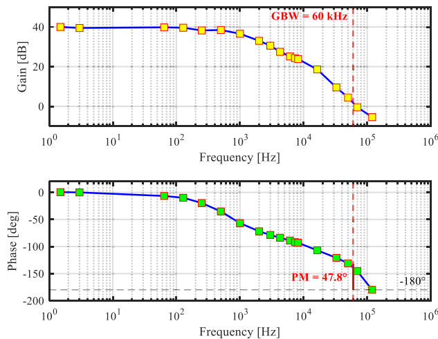
FIGURE 8. Bode plots of the differential voltage amplification of the FI-DIGOTA.
