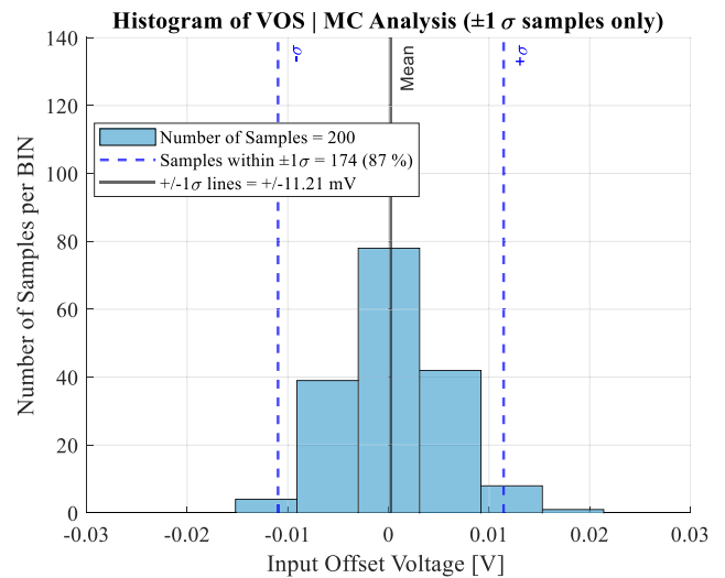
FIGURE 9. Distribution of the input offset voltage of the FI-DIGOTA in UGFB configuration based on 200 samples Monte-Carlo simulations including process variations and mismatch.
