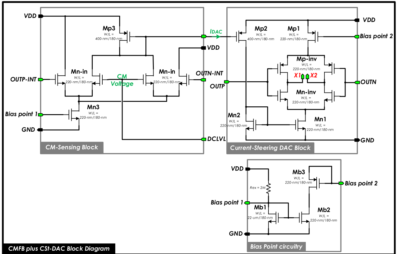
FIGURE 6. CMFB block diagram including CM-mode sensing, current-steering DAC, and bias circuitry.
