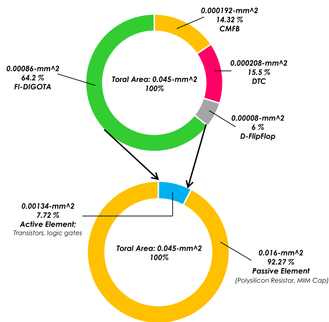
FIGURE 15. Area distribution of the whole system in percentage.
