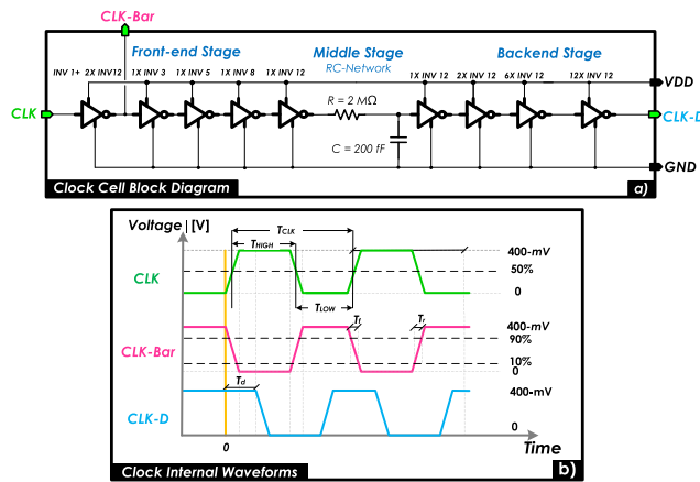
FIGURE 5. a) Clock generation block b) Internal clock timing waveforms.
