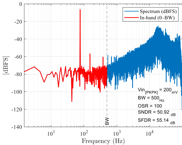
FIGURE 11. Output spectrum of the first-order \Sigma\Delta modulator for a 76.3 Hz sine-wave with the input peak-to-peak amplitude of 200 mV.
