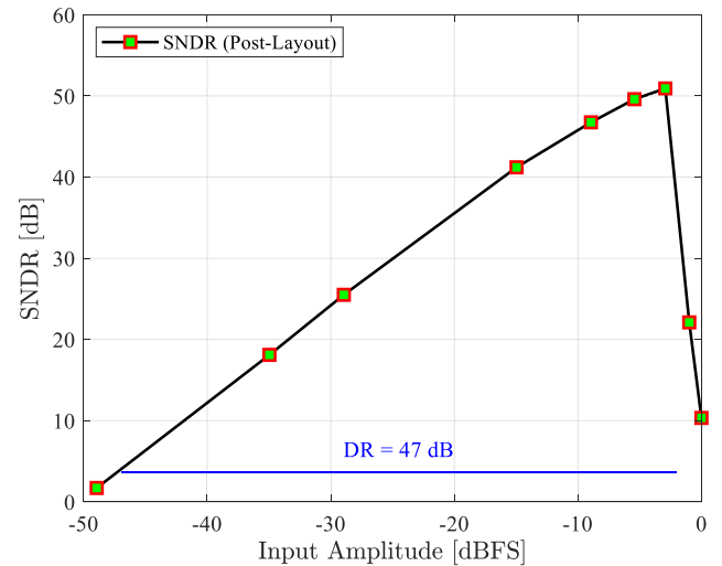
FIGURE 13. SNDR versus input amplitude of the first-order \Sigma\Delta modulator for a sine-wave input signal from post-layout simulation.
