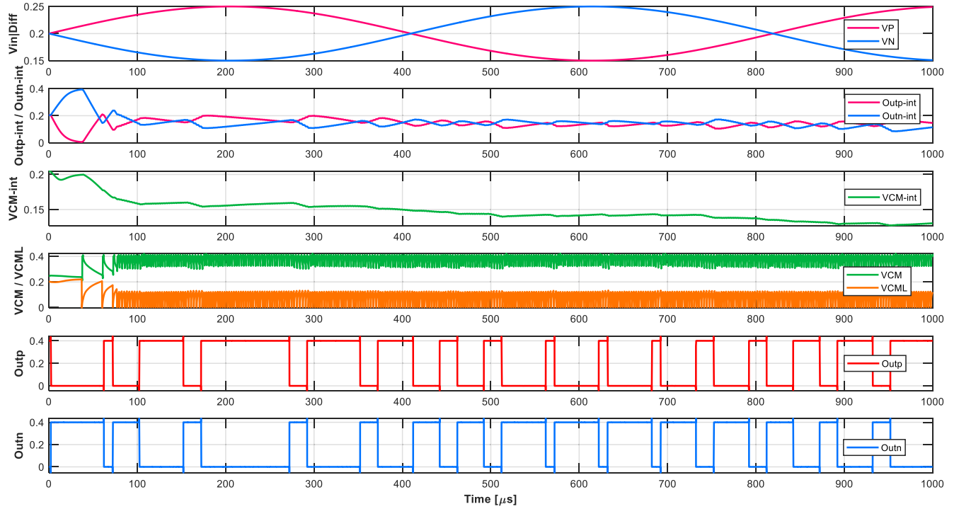
FIGURE 4. Time-domain waveforms of the proposed FI-DIGOTA under differential sinusoidal excitation. From top to bottom: differential input signal ( V_{inDiff} ), differential integrator output voltages ( V_{Outp.int} and V_{Outn.int} ), resulting integrator output common-mode voltage ( V_{CM.int} ), common-mode control voltages of the FI-DIGOTA ( V_{CM} and V_{CMCL} ), and corresponding digital output signals.
