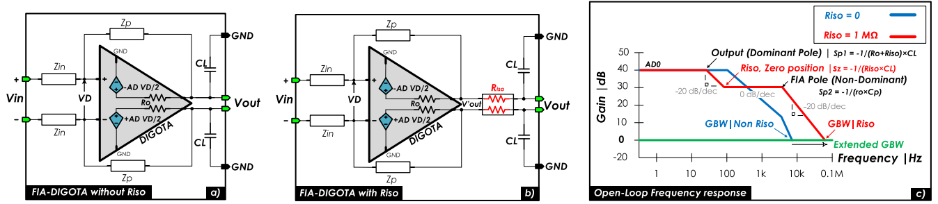
FIGURE 2. a,b) Frequency compensation circuit with/without attenuation resistor ( R_{iso} ) on closed-loop gain configuration, c) bode gain plot for with(out) attenuation resistor in open-loop gain configuration.
