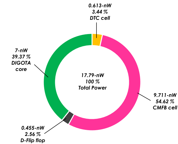
FIGURE 14. Power distribution of the whole system in percentage.
