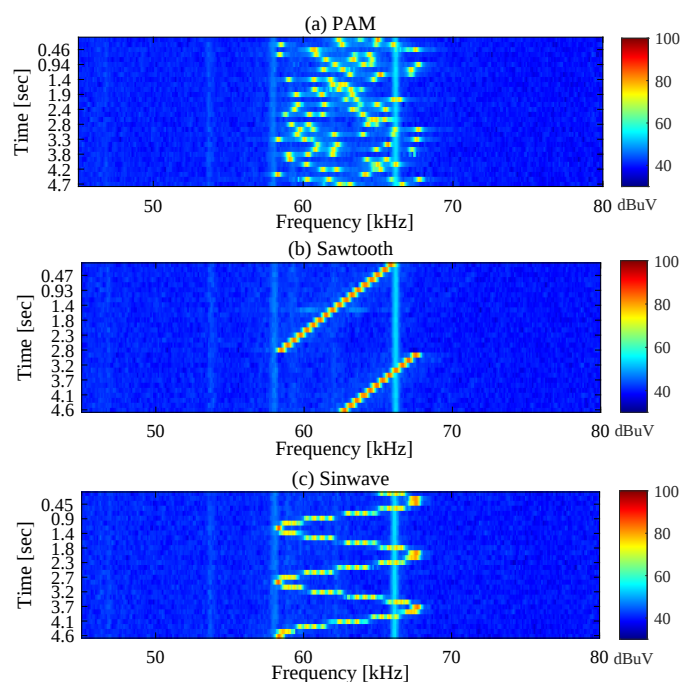
Figure 4. The voltage spectrum measured from the PLC circuit side in the case of using various profiles of \varepsilon(t) at f_m = 0.3 and \alpha = 0.15 .
