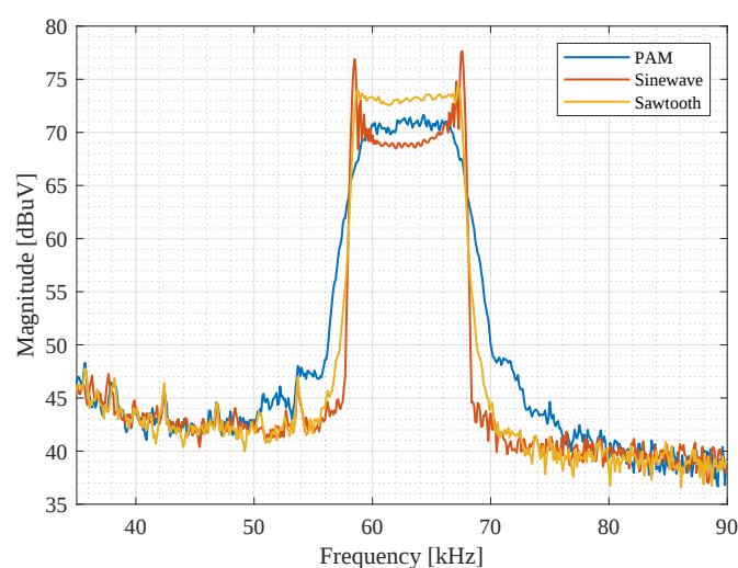
Figure 3. The voltage spectrum measured from the PLC circuit side in the case of using various profiles of \varepsilon(t) and constant \alpha .
