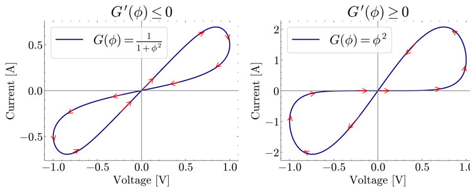
FIGURE 3 | Simulated I vs. V curves of two distinct periodically-forced memristors with the indication of the direction of motion of the point trajectory along them over time, as induced by different memductance trends: decreasing G(\phi) (a) and increasing G(\phi) (b). A sinusoidal voltage input of unitary amplitude is applied across the ideal memristor in both cases.
