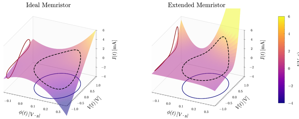
FIGURE 2 | Three-dimensional (I, V, \phi) representations of the ideal (left) and extended (right) memristor models under the sinusoidal excitation v(t) = A \sin(2\pi f t) with A = 1 V and f = 1 Hz. For each model, the semi-transparent plasma surface visualizes the full current domain obtained by evaluating the constitutive equation over the (\phi, V) meshgrid. The black dashed curve denotes the actual system trajectory generated by the applied input, while the dark-red and navy curves represent its projections onto the (I, V) and (\phi, V) planes, respectively. In the ideal case, the current collapses onto a single flux-dependent manifold I = G(\phi)V , here illustrated using G(\phi) = \beta \cdot \phi^2 with \beta = 0.04 , resulting in symmetric lobes. Conversely, the extended memristor produces a fully shaped and non-collapsing (I, V, \phi) domain, enabling asymmetric and device-specific behaviors; the illustrative memductances G_+(\phi, V) = 3\beta \cdot \phi^2 \cdot V^2 and G_-(\phi, V) = \beta \cdot \phi^4 are used solely to demonstrate this generalized framework. \phi is obtained as the time integral of the voltage and it has initial condition \phi(0) = 0 .
