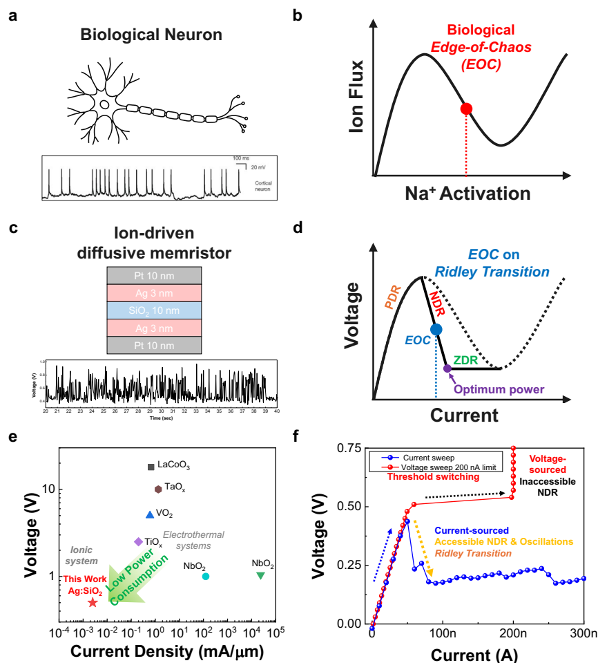
Fig. 1 | Edge of chaos dynamics in ion-driven diffusive memristors inspired by biological neurons. a Schematic of a biological neuron showing periodic spiking behavior. Spiking data reproduced from ref. 48 under a Creative Commons Attribution 3.0 license, https://creativecommons.org/licenses/by/3.0/ . No changes were made. b Conceptual illustration of the quasi-static nonlinear ionic response in a biological neuron. The ordinate represents the \text{Na}^+ ionic flux (or equivalently, the \text{Na}^+ -mediated ionic current) as a function of \text{Na}^+ channel activation. The EOC operating point corresponds to a locally active but stable regime, often associated with regions of negative differential resistance (NDR), where small perturbations can be strongly amplified. c Schematic of an Ag:SiO 2 film diffusive memristor illustrating ionic drift-diffusion through a conductive channel within a vertically
