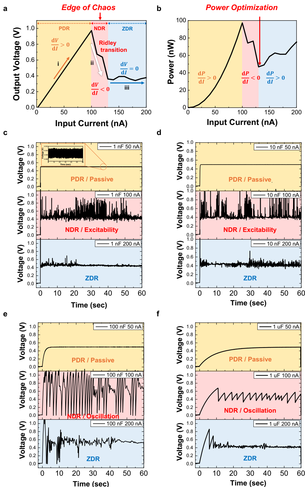
Fig. 2 | Electrical characterization of a diffusive memristor. a Quasi-static DC V-I characteristics of the diffusive memristor (current sweep rate 500 \text{ nA s}^{-1} ) without an intentionally added external parallel capacitor (i.e., only intrinsic and stray capacitances of \sim 10 \text{ pF} are present), highlighting regimes of positive differential resistance (PDR), negative differential resistance (NDR), and zero differential resistance (ZDR), depending on the applied current. b Power vs. current corresponding to (a) , showing that the Ridley transition significantly reduced the power dissipation and thus the entropy production in the device. c, d Time-dependent voltage ( V-t )
