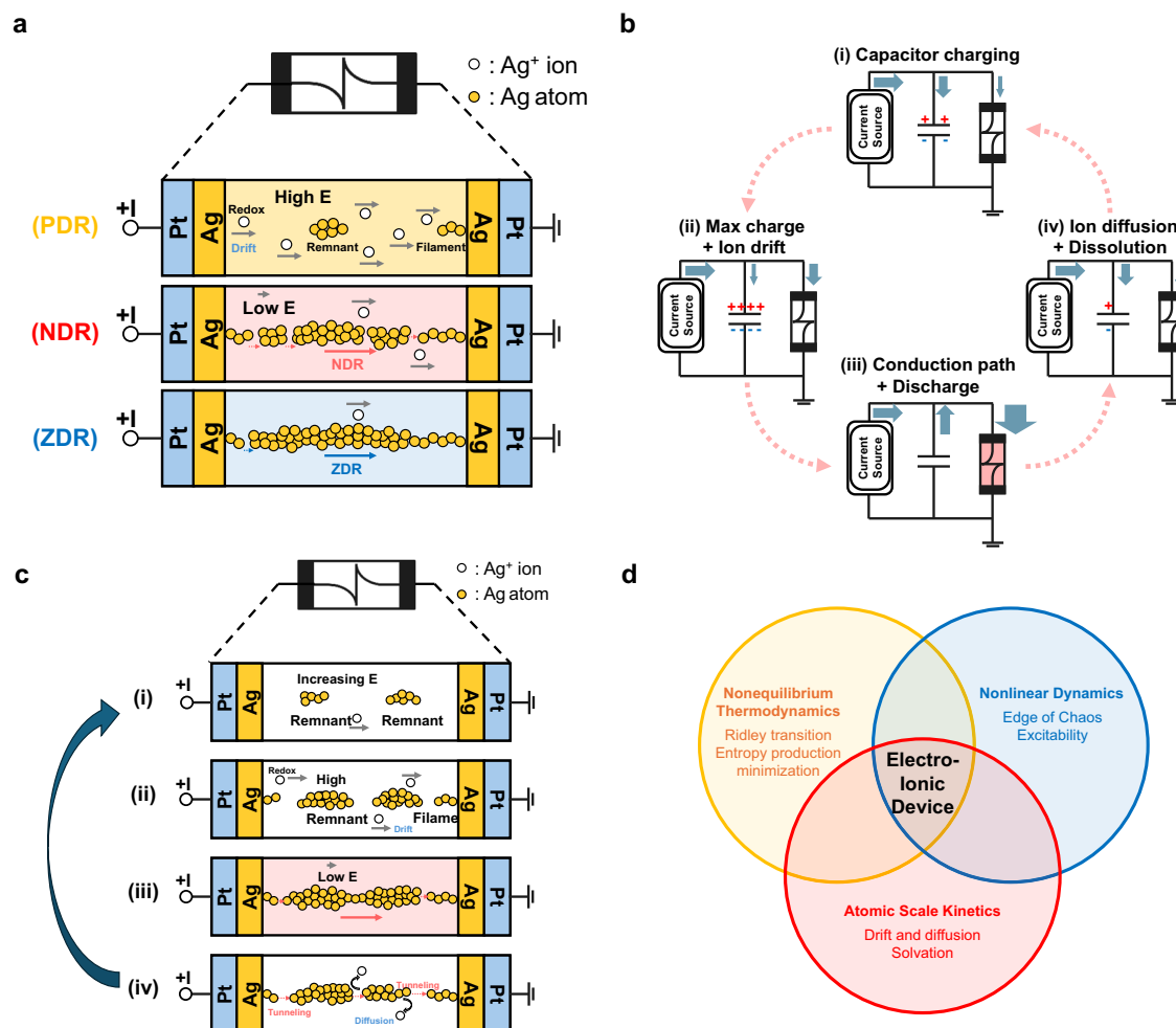
Fig. 4 | Atomic-scale mechanism of edge of chaos dynamics in diffusive memristors informed by compact model simulations. a Schematic illustration of atomic-scale steady-state PDR, NDR, and ZDR phenomena in a diffusive memristor. b Circuit-level depiction of the oscillatory mechanism under current-controlled operation with an external capacitor, illustrating the four key stages. c Schematic
