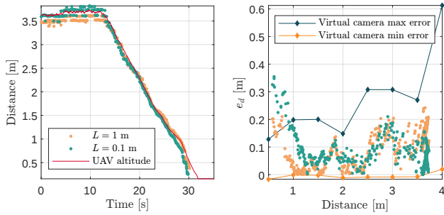
Fig. 8. Visual navigation performance in RoboticsXR framework with real-time UAV motion in a realistic mountain environment.
