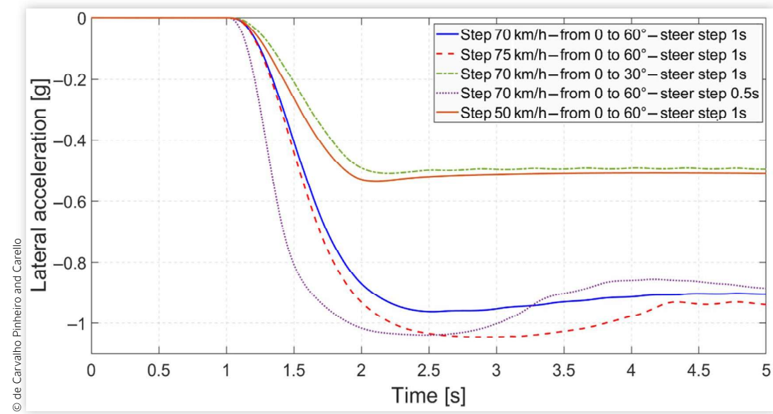
FIGURE A.5 FOSM low-pass control—Step steering vehicle response.
