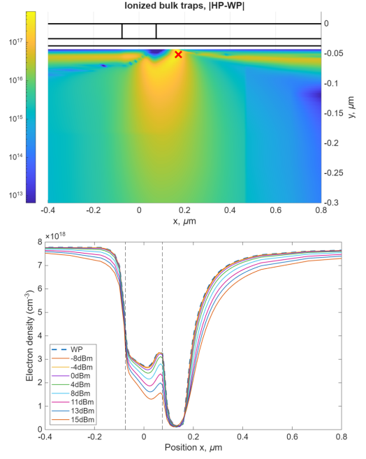
Fig. 5: Class A DC behavior. Top: difference of occupied traps DC component at available input power P_{av} = 15 dBm (HP) and at the DC working point (WP). The “x” represents the point investigated in Figs. 6-7. Bottom: cross section of the electron density in the channel, 1 nm below the AlGaN/GaN interface, as a function of the available power.
