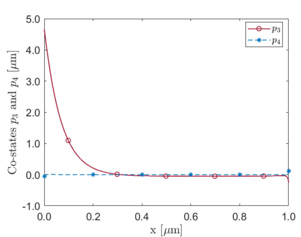
(D) Spatial distribution of the co-states p_3 and p_4 .
