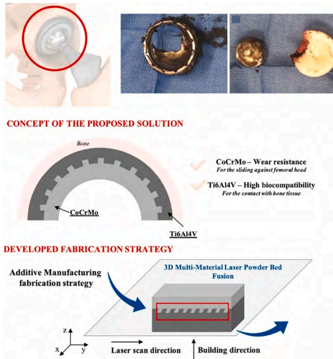
Fig. 26. Example of biomedical application of mechanical interlocking structures. Acetabular cup concept combining dissimilar metals through planar-based macro-lattices, enhancing mechanical performance at the interface. Reprinted from [88], Copyright (2023), with permission from Elsevier.
