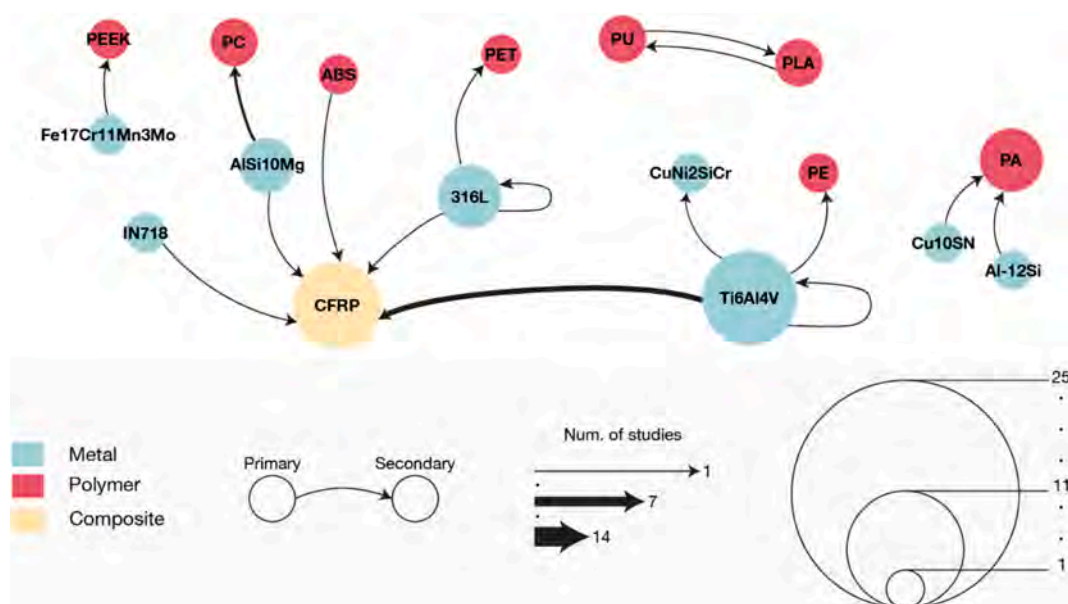
Fig. 17. Bubble map of material combinations for micro-features. Arrow direction indicates the interlocking configuration: the tail corresponds to the primary material, while the arrowhead points to the secondary material. Line thickness scales with the number of studies for a given combination. Node size is proportional to the number of citations of each material in the literature.
