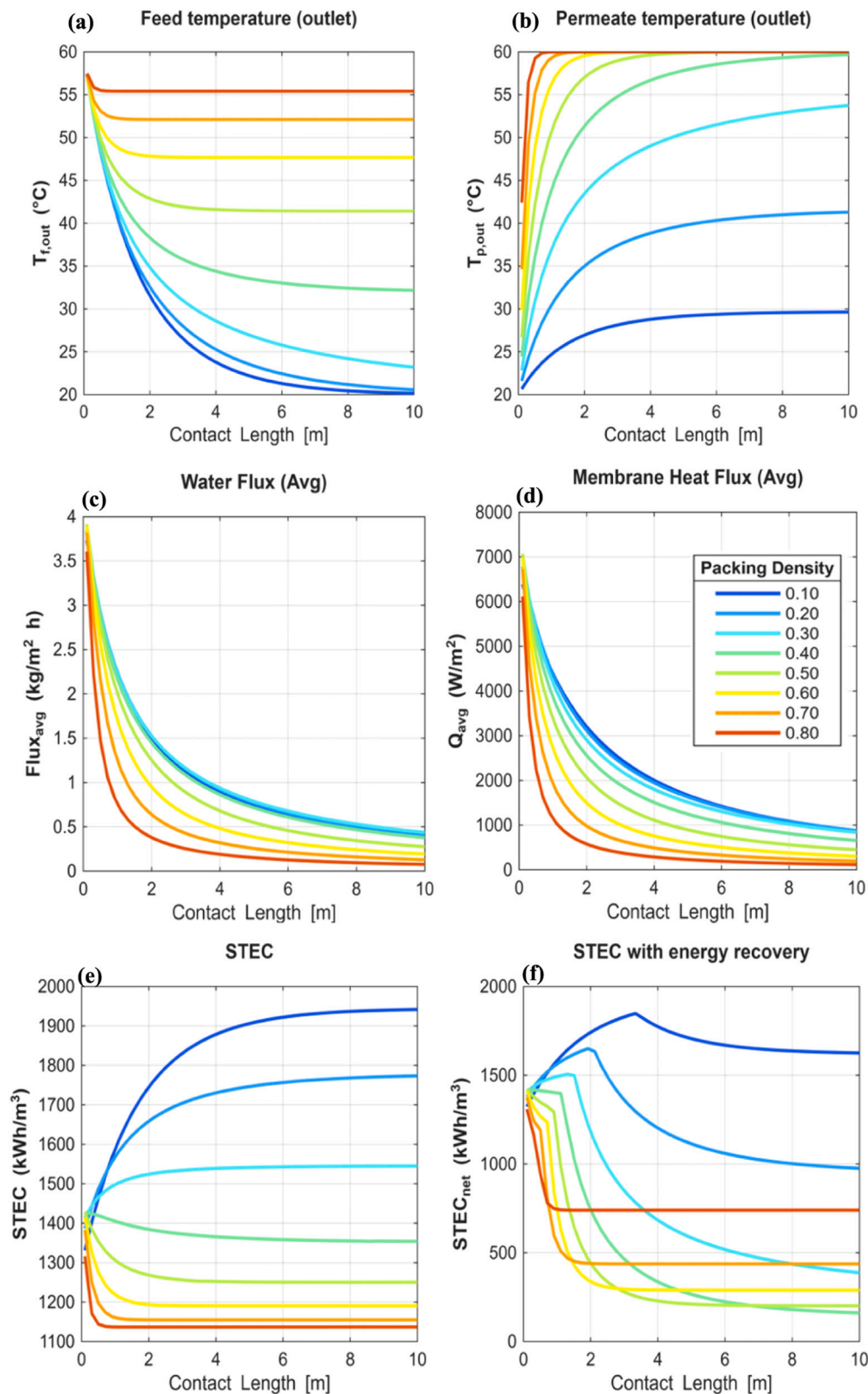
Fig. 3. Effect of contact length on various parameters at different values of packing densities ranging from 0.1 to 0.8. The operating conditions were set at: inlet feed temperature 60 °C, inlet permeate temperature 20 °C, inlet feed velocity 0.125 m/s and inlet permeate velocity 0.025 m/s.
