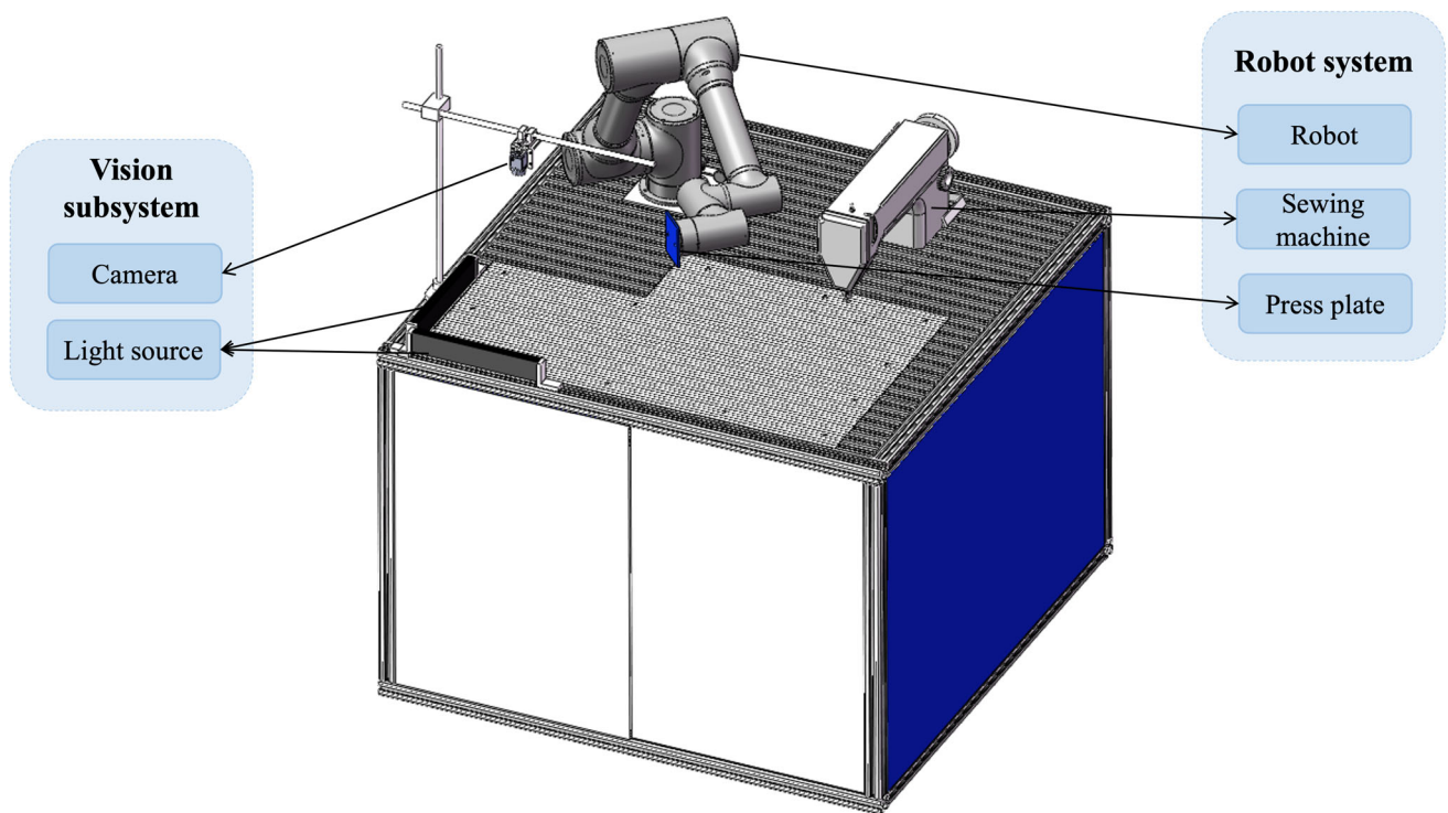
Fig. 1 Overall architecture of the vision-based sewing robot system
